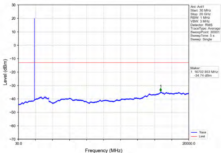
Band2_1.4MHz_16QAM_HCH_1909.3MHz_RB_1_0_NTNV
