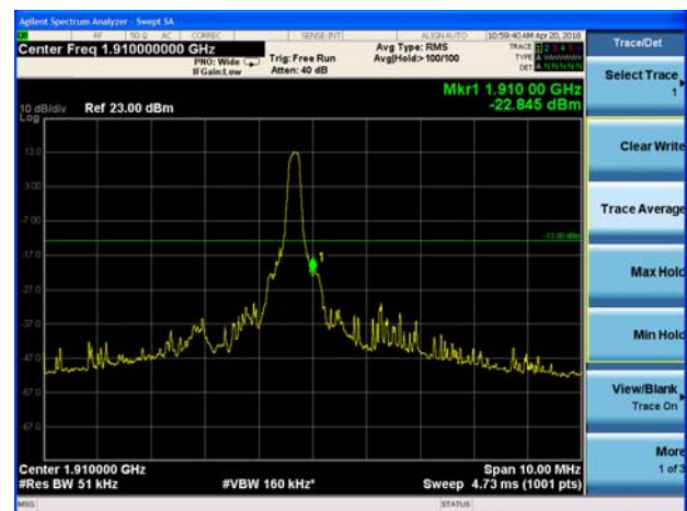
LTE Band 2 5MHz 16QAM 100%RB CH-High
