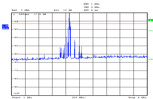
LTE Band 2 1.4MHz CH-Low 1GHz~3GHz
