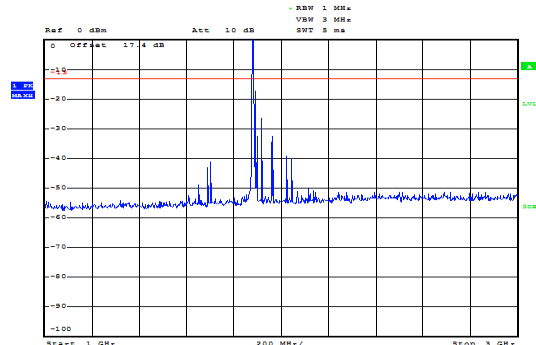
LTE Band 2 1.4MHz CH-Middle 1GHz~3GHz
