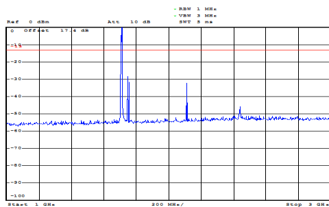
LTE Band 4 1.4MHz CH-Low 1GHz~3GHz
