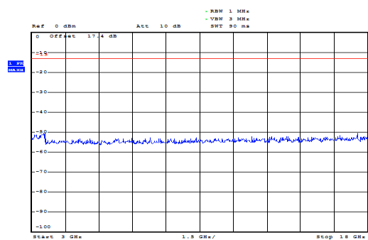
LTE Band 4 1.4MHz CH-Middle 3GHz~18GHz
