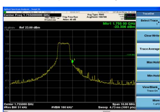
LTE Band 4 16QAM 5MHz CH-High, 100%RB
