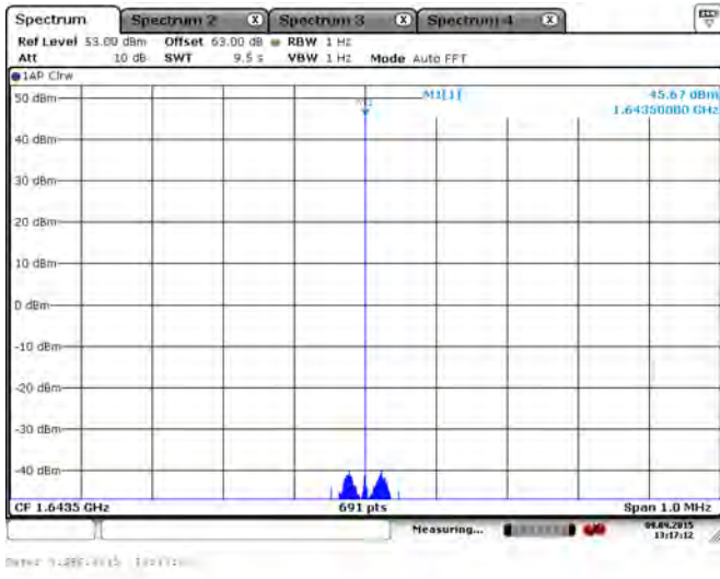
Illustration 65: Carrier frequency: 40V power supply.
