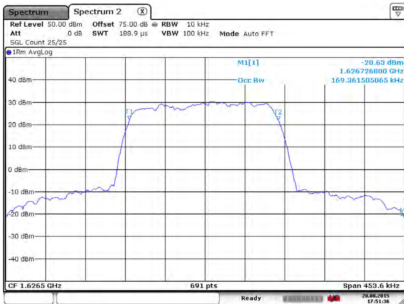
Illustration 55: Occupied Bandwidth.
