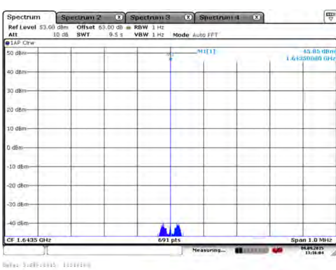
Illustration 63: Carrier frequency: 16V power supply.
