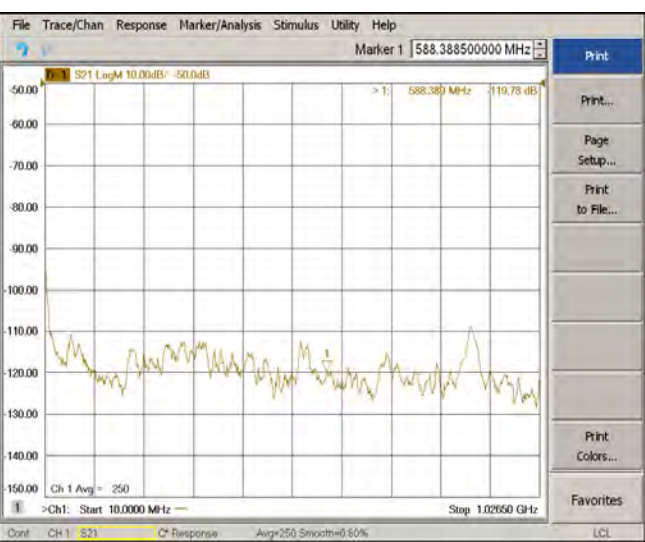
Illustration 66: 10MHz - 1026.5MHz
