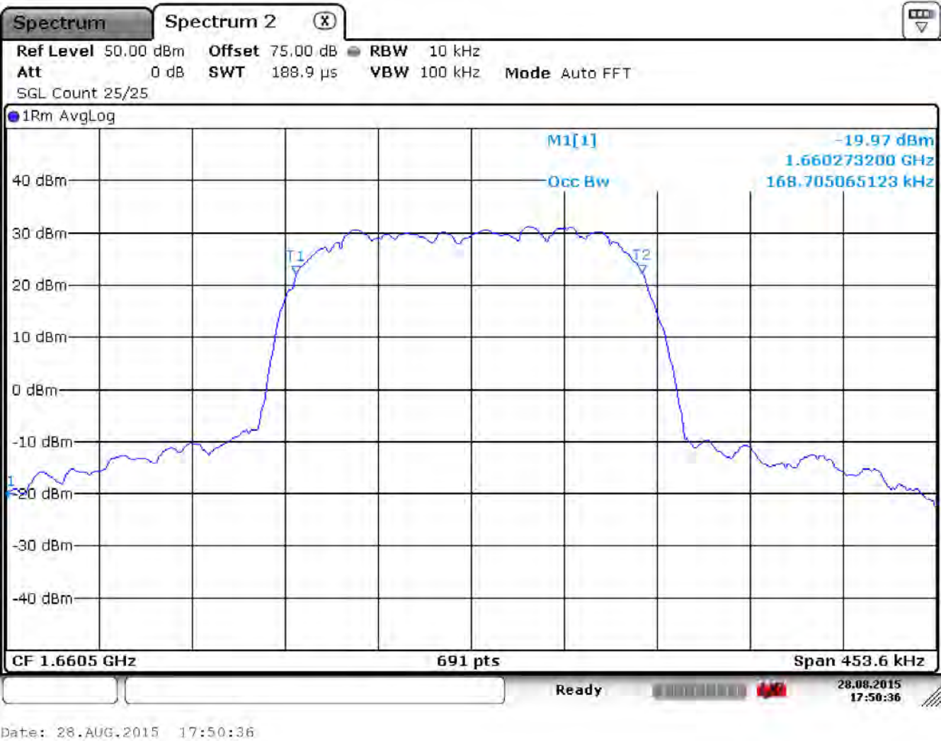
Illustration 54: Occupied Bandwidth.
