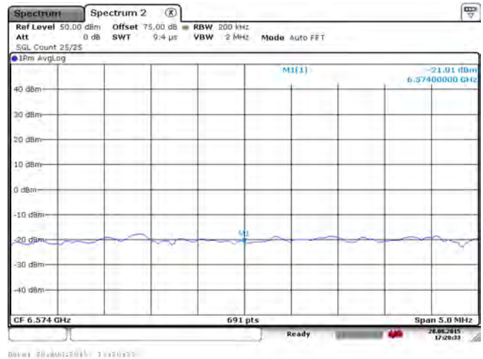
Illustration 18: Spectrum @ 4th harmonic frequency.
