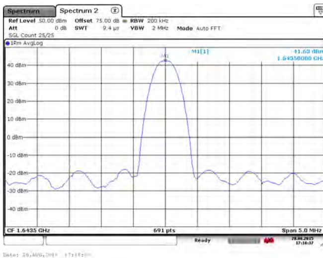
Illustration 17: Spectrum @ fundamental frequency.
