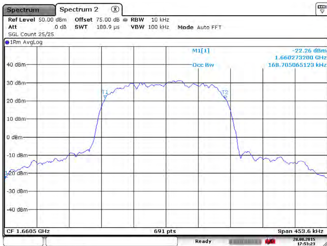
Illustration 57: Occupied Bandwidth.
