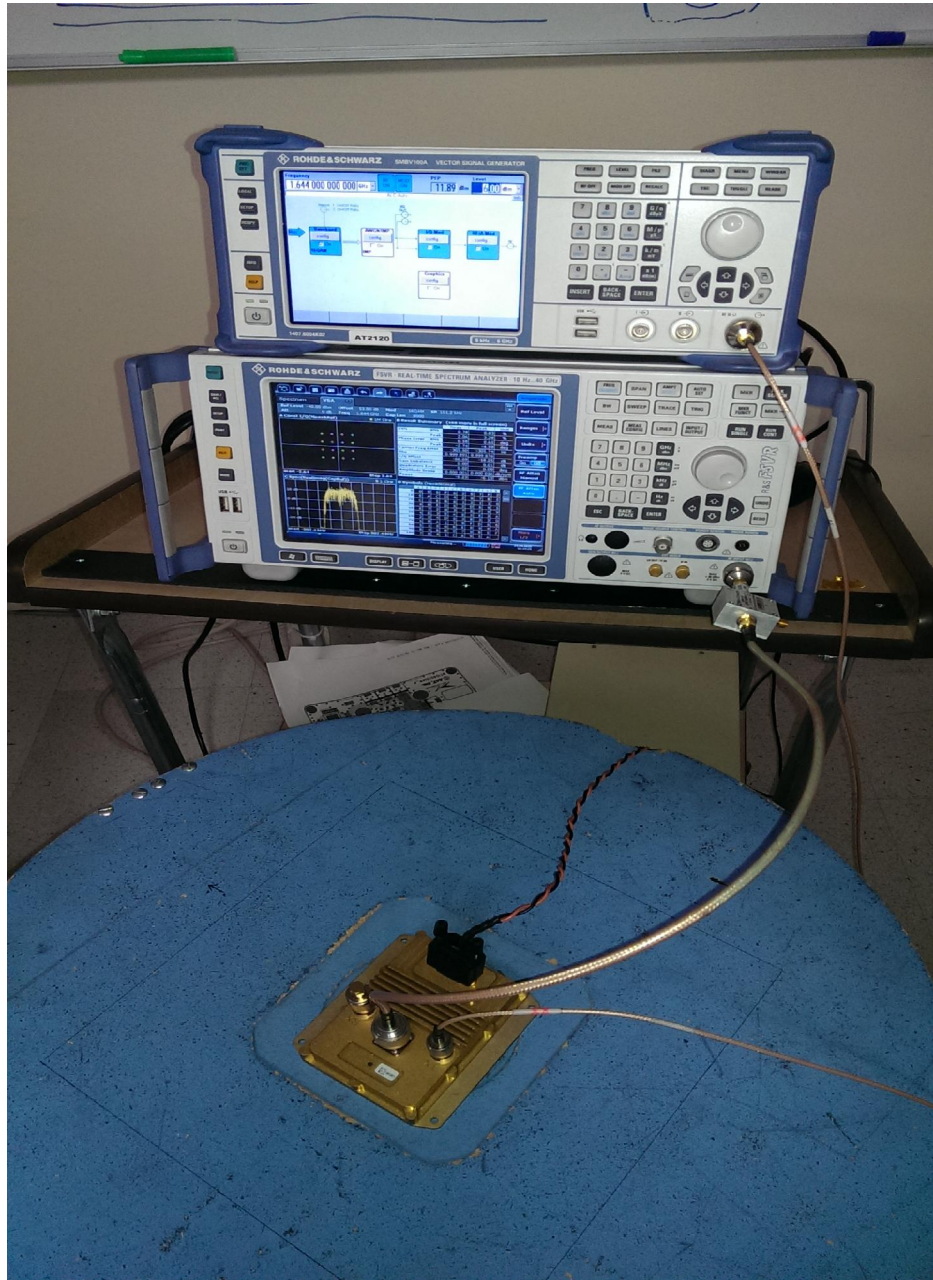
Illustration &#. Conducted Emissions Test Setup.
