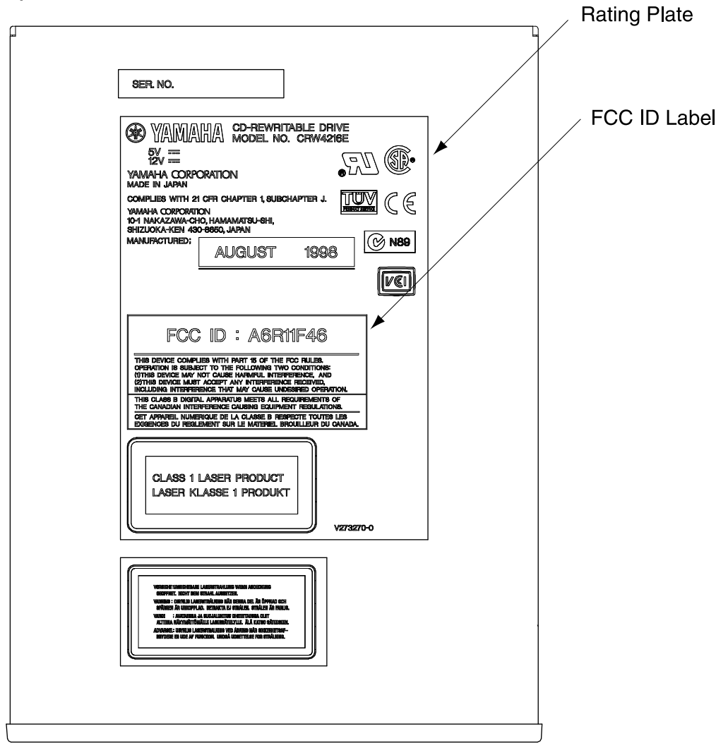
Top View of EUT
