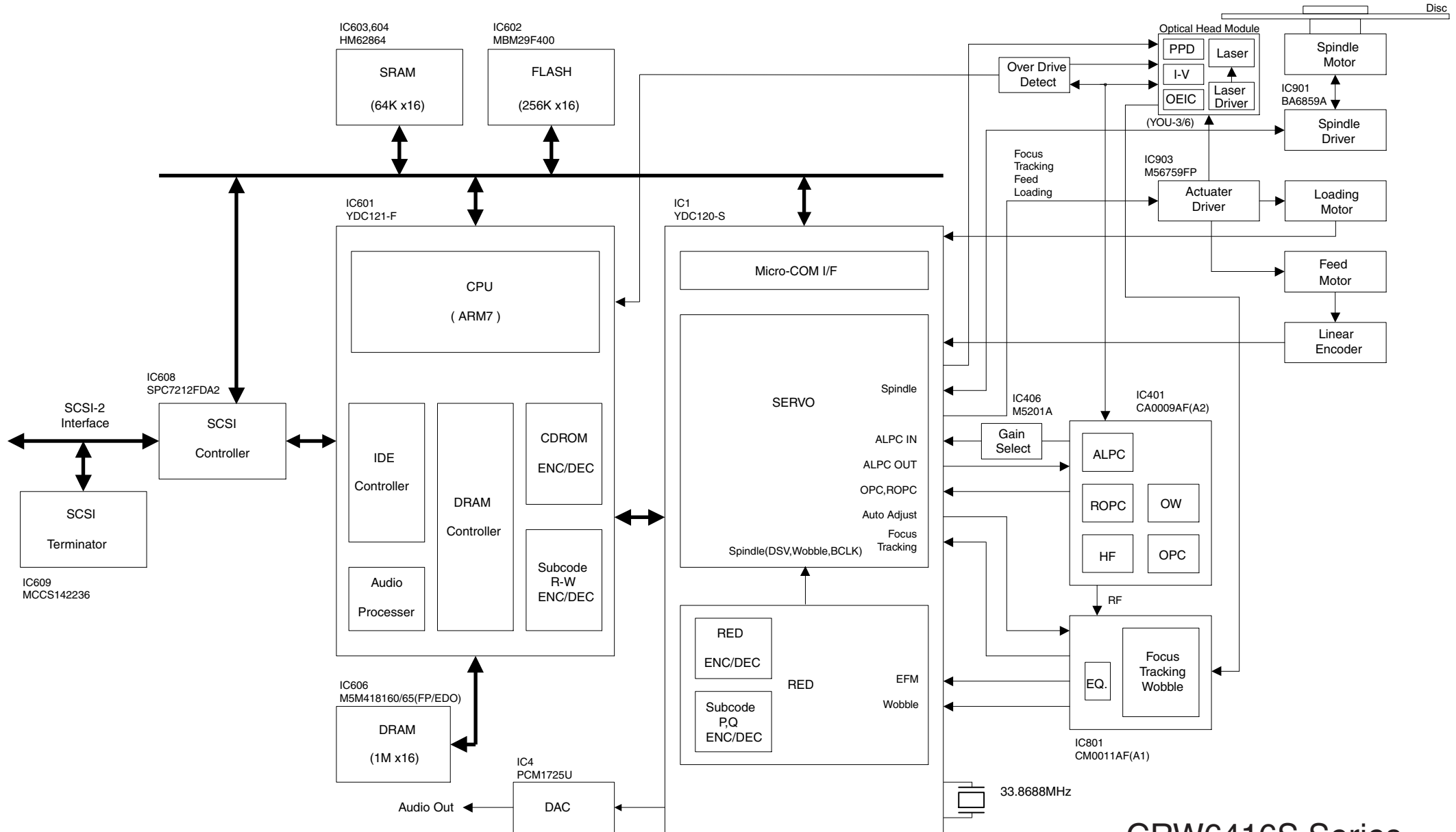
CRW6416S Series Block Diagram
