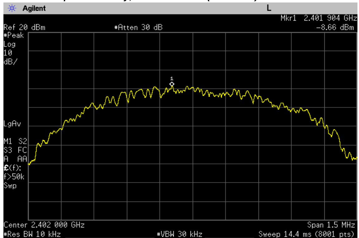
Peak Power Spectral Density, Lowest Channel (2 402 MHz)
