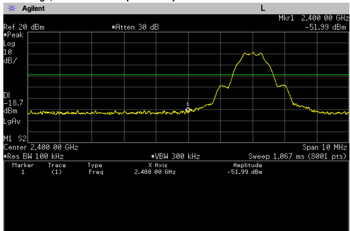
Band Edge, Lowest Channel (2 402 MHz)
