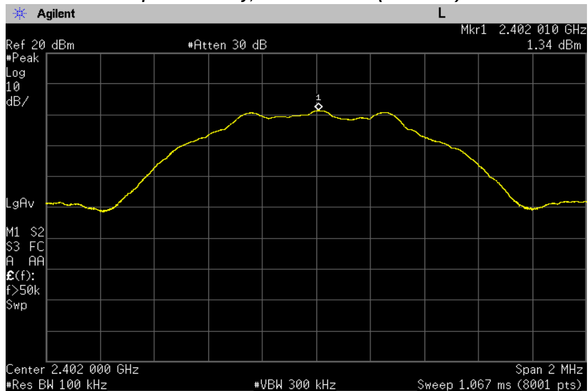
Reference Power Spectral Density, Lowest Channel (2 402 MHz)
