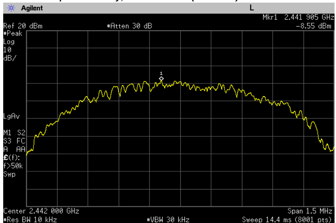
Peak Power Spectral Density, Middle Channel (2 442 MHz)
