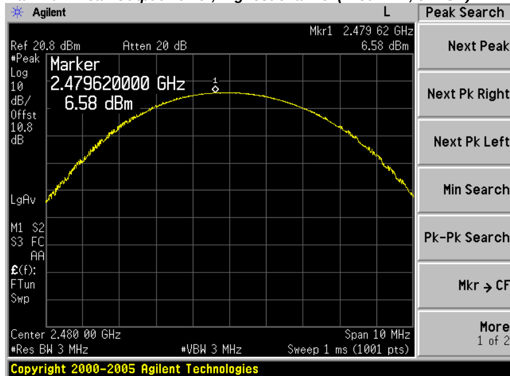
Maximum Peak Output Power, Highest channel (2480 MHz, 8DPSK)
