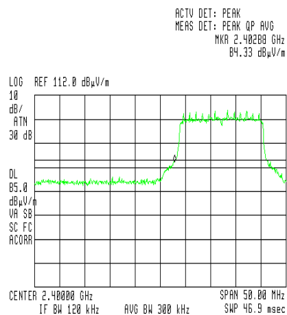
Figure 100 — Channel 1, 6Mbps
