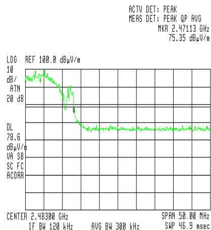
Figure 109 — Channel 11, 130Mbps
