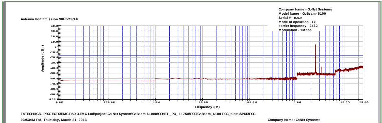
Figure 90 – Channel 11 , 1Mbps
