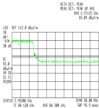
Figure 107 — Channel 11, 54Mbps
