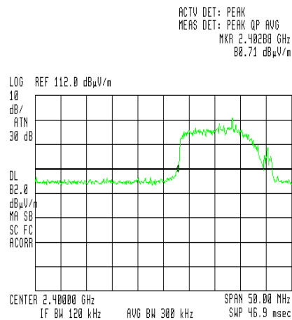
Figure 103 — Channel 1, 130Mbps
