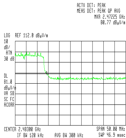
Figure 108 — Channel 11, 6.5Mbps
