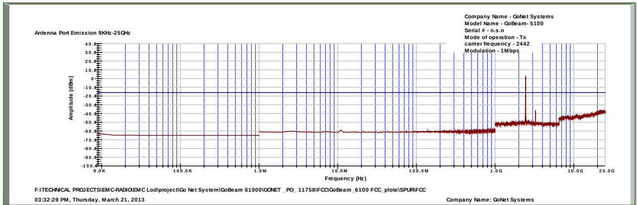
Figure 84 – Channel 6 , 1Mbps
