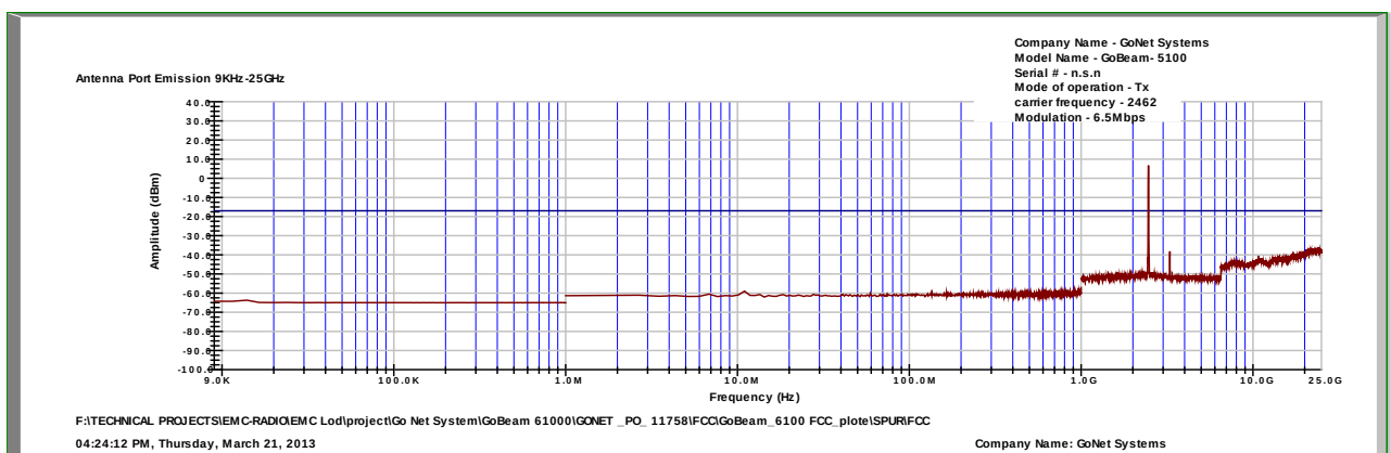
Figure 94 – Channel 11 , 6.5Mbps
