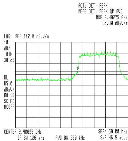
Figure 102 — Channel 1, 6.5Mbps
