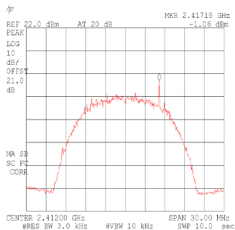
Figure 131 - Channel 1 , 130Mbps
