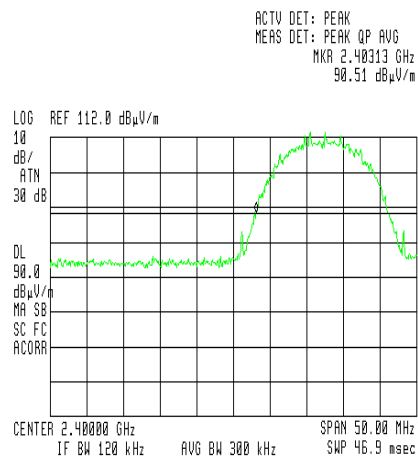
Figure 99 — Channel 1, 11Mbps
