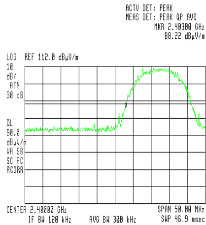
Figure 98 — Channel 1, 1Mbps
