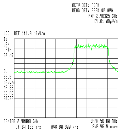
Figure 101 — Channel 1, 54Mbps
