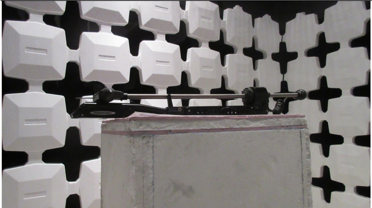
Radiated Testing, Table Setup #1
