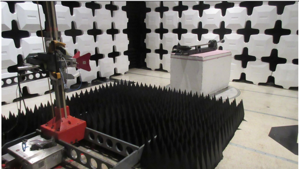
Radiated Testing, Above 1 GHz #1
