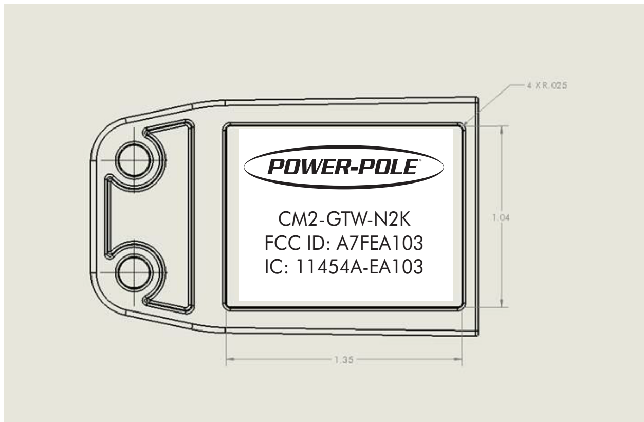
Bottom view of the NMEA2K Gateway
