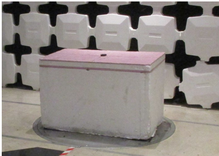
Radiated Testing, Table Setup #1
