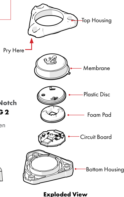
Exploded View
