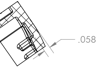
SECTION E-E SCALE 2 : 1
