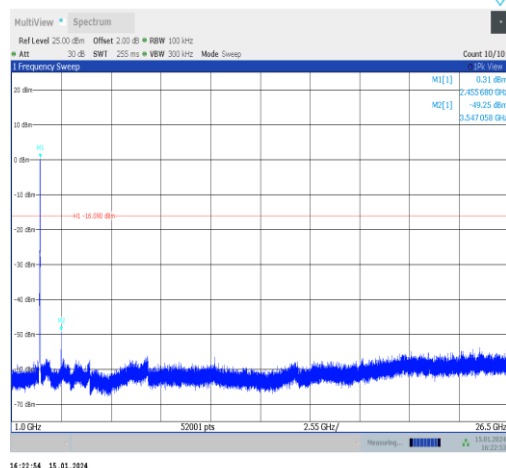
11n40SISO-Ant1-2452-1000~26500-PASS
