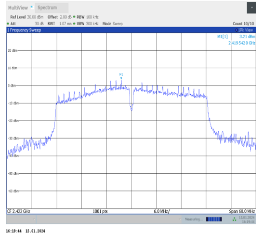
11n40SISO-Ant1-2422-0~Reference-PASS
