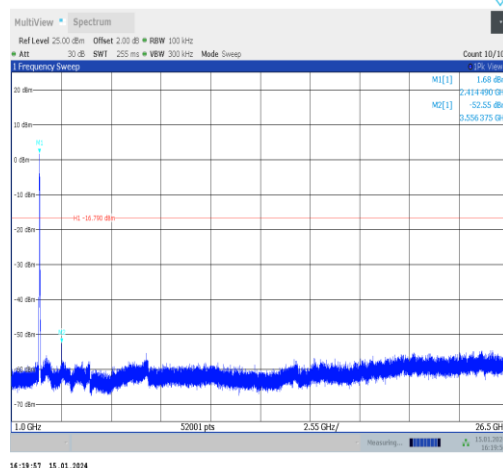
11n40SISO-Ant1-2422-1000~26500-PASS
