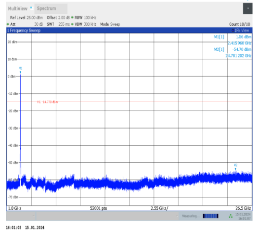
11g-Ant1-2412-1000~26500-PASS
