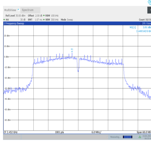
11n40SISO-Ant1-2452-0~Reference-PASS
