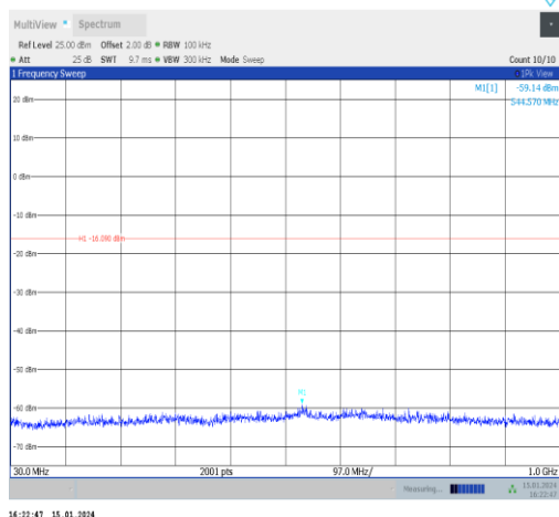
11n40SISO-Ant1-2452-30~1000-PASS
