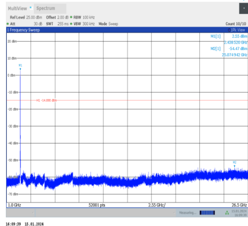
11n20SISO-Ant1-2437-1000~26500-PASS
