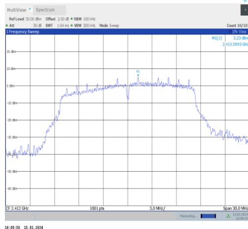
11g-Ant1-2412-0~Reference-PASS
