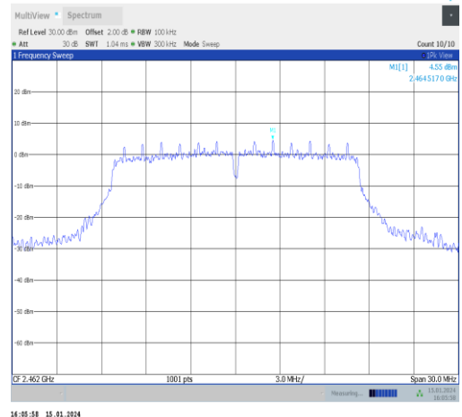
11g-Ant1-2462-0~Reference-PASS
