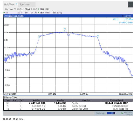
11n40SISO-Ant1-2452
