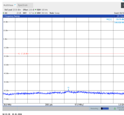
11n40SISO-Ant1-2437-30~1000-PASS
