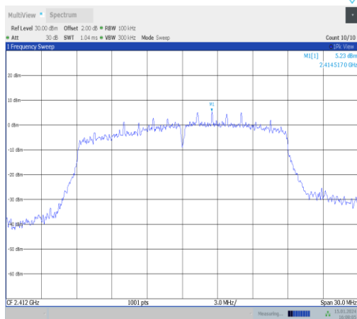
11n20SISO-Ant1-2412-0~Reference-PASS
