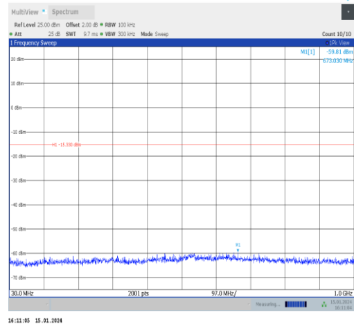
11n20SISO-Ant1-2462-30~1000-PASS
