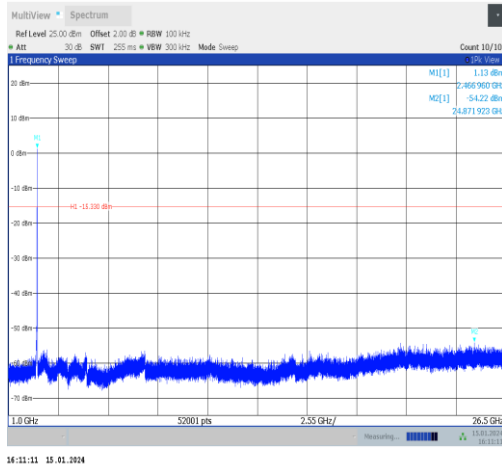
11n20SISO-Ant1-2462-1000~26500-PASS
