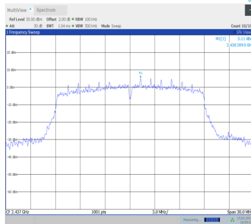
11n20SISO-Ant1-2437-0~Reference-PASS
