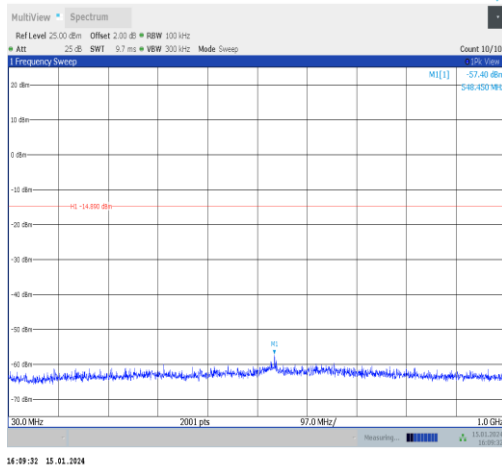
11n20SISO-Ant1-2437-30~1000-PASS
