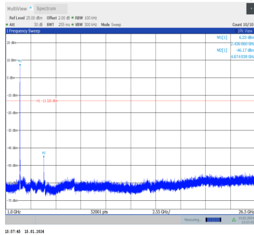
11b-Ant1-2437-1000~26500-PASS
