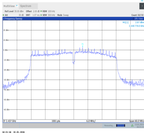
11n40SISO-Ant1-2437-0~Reference-PASS
