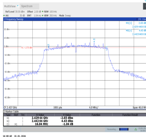
11n20ISO-Ant1-2437-PASS
