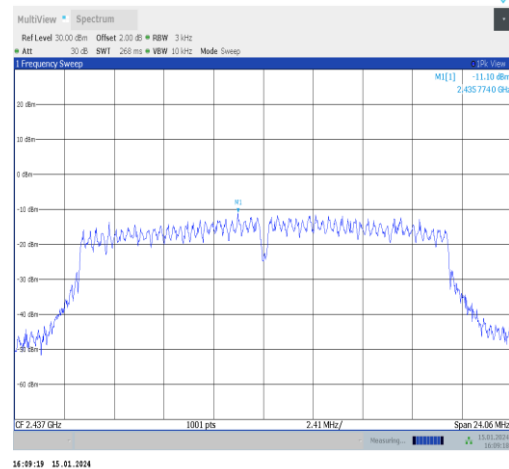
11n20ISO-Ant1-2437-PASS
