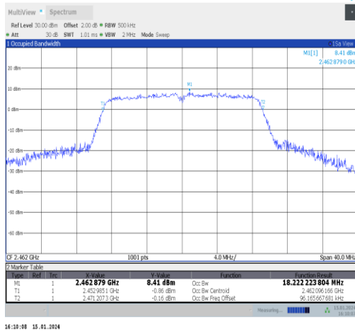
11n20SISO-Ant1-2462
