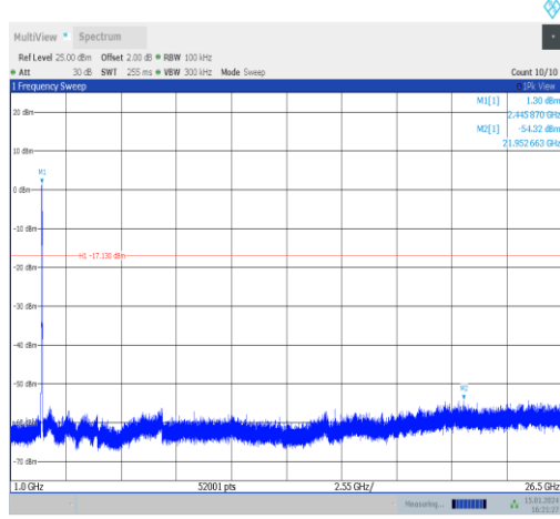
11n40SISO-Ant1-2437-1000~26500-PASS
