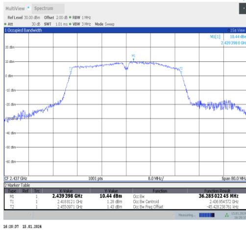
11n40SISO-Ant1-2437
