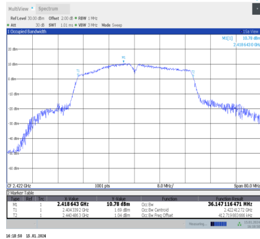
11n40SISO-Ant1-2422
