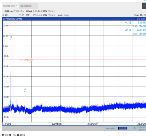
11b-Ant1-2462-1000~26500-PASS
