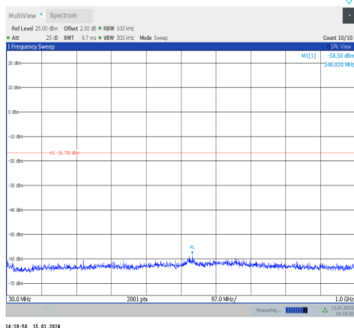
11n40SISO-Ant1-2422-30~1000-PASS
