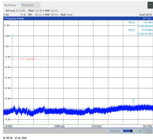
BLE_1M-Ant1-2440-1000~26500-PASS
