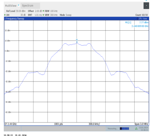
BLE_1M-Ant1-2440-0~Reference-PASS
