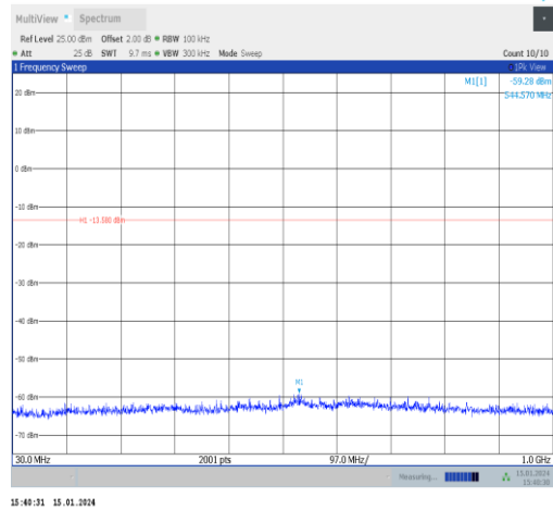
BLE_1M-Ant1-2480-30~1000-PASS
