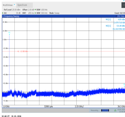
BLE_1M-Ant1-2480-1000~26500-PASS
