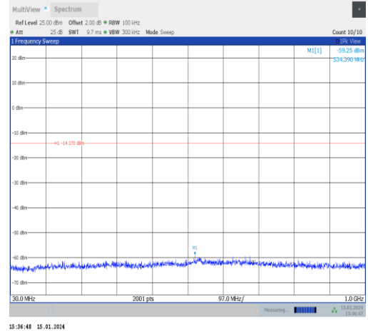
BLE_1M-Ant1-2402-30~1000-PASS
