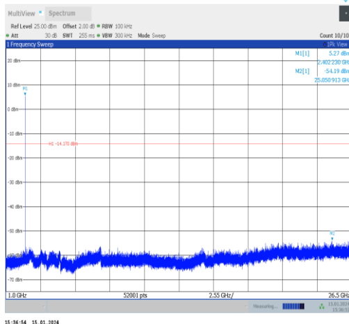
BLE_1M-Ant1-2402-1000~26500-PASS
