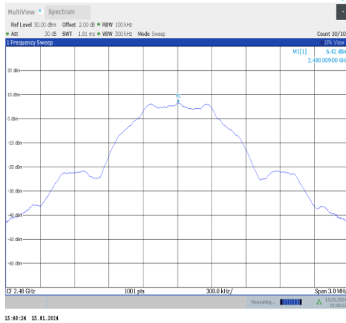
BLE_1M-Ant1-2480-0~Reference-PASS
