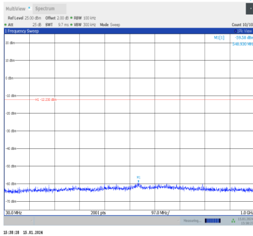
BLE_1M-Ant1-2440-30~1000-PASS
