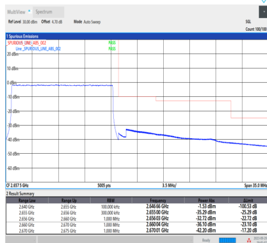
Band41_15MHz_QPSK_41165_75RB#0
