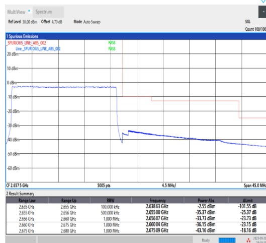
Band41_20MHz_QPSK_41140_100RB#0
