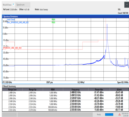
Band41_15MHz_QPSK_40315_1RB#0
