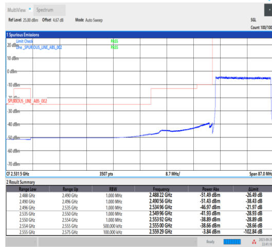
Band41_20MHz_QPSK_40340_100RB#0
