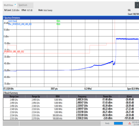
Band41_15MHz_QPSK_40315_75RB#0
