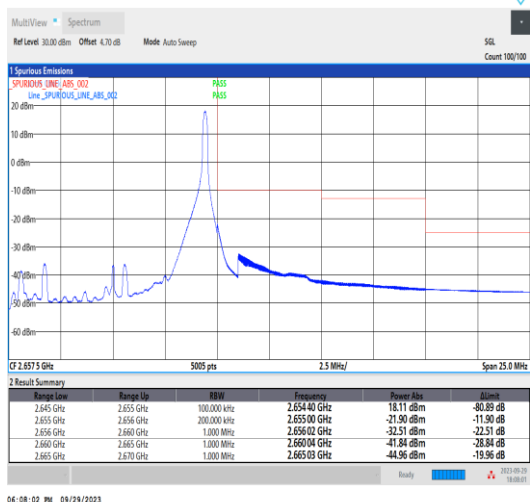
Band41_10MHz_QPSK_41190_1RB#49
