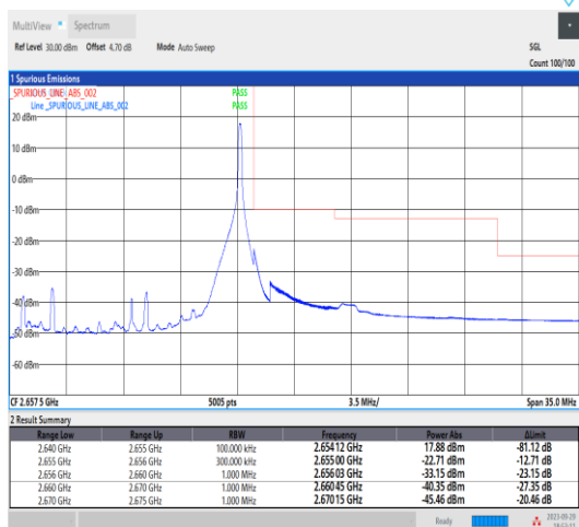
Band41_15MHz_QPSK_41165_1RB#74
