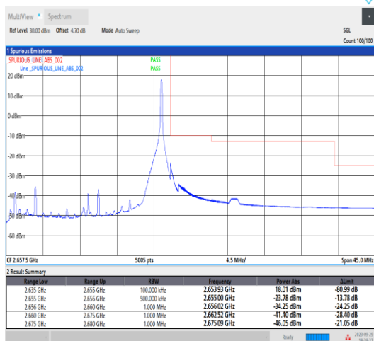
Band41_20MHz_QPSK_41140_1RB#99
