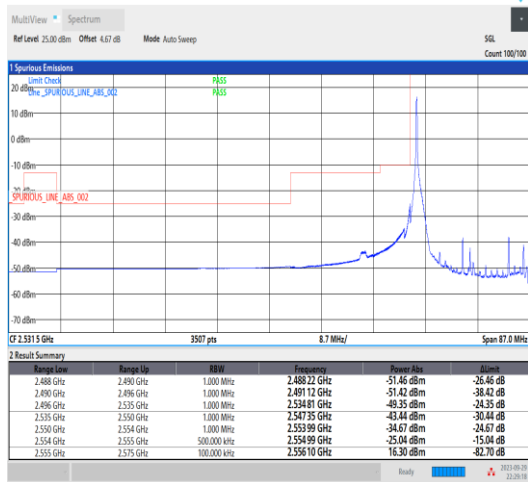
Band41_20MHz_QPSK_40340_1RB#0
