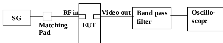
Figure 6. Picture sensitivity
