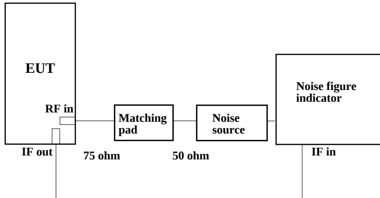
Figure 7. Noise figure
