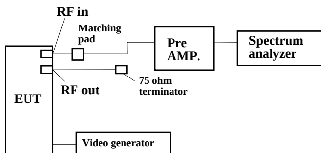
Figure 5. Antenna transfer switch
