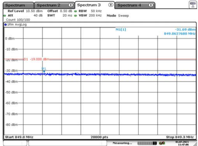
Right Side-WCDMA-Above AGC
