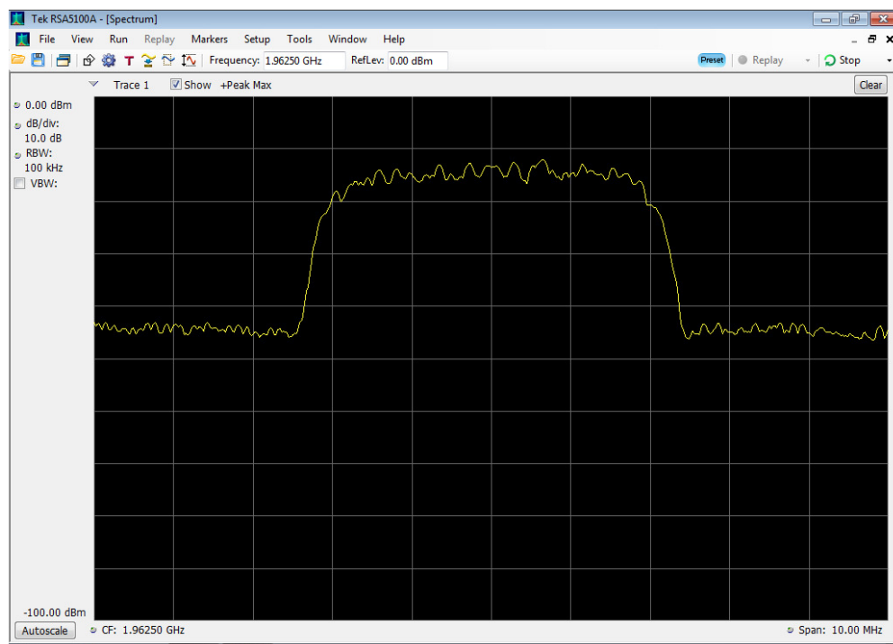
WCDMA output_1930-1995 MHz
