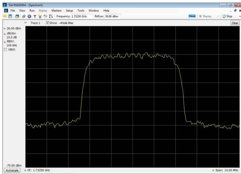
WCDMA output_1710-1755 MHz
