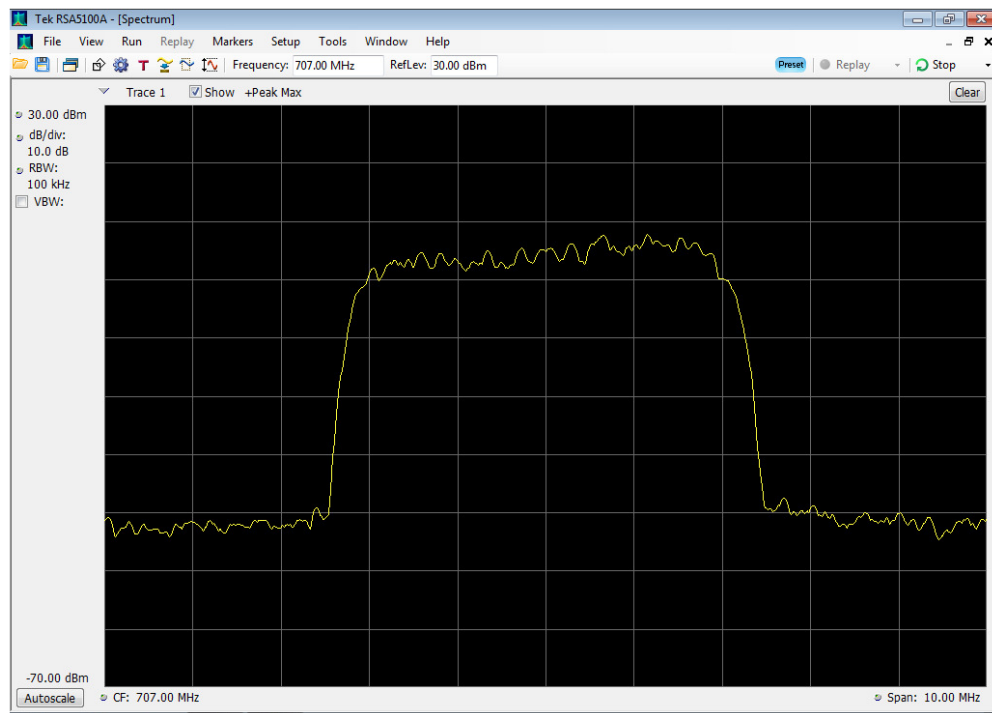
WCDMA output_698 - 716 MHz
