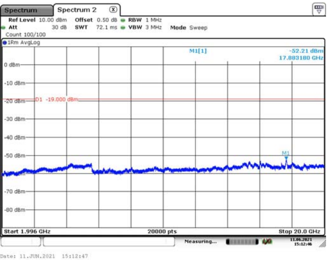
PCS Band-3
