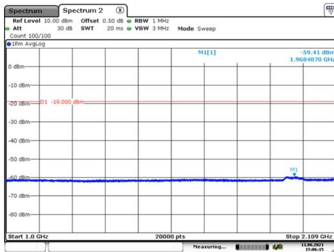
AWS Band-2
