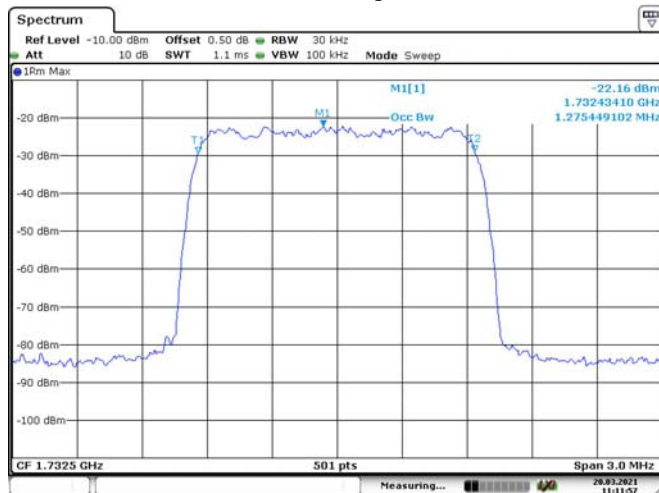
CDMA-Input
