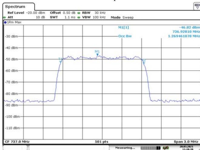
CDMA-Input
