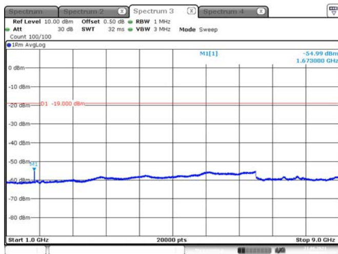
Cellular Band-3
