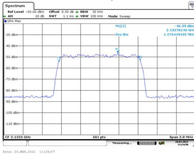
WCDMA-Input
