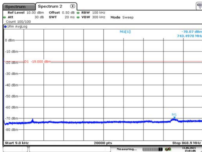
Cellular Band-1
