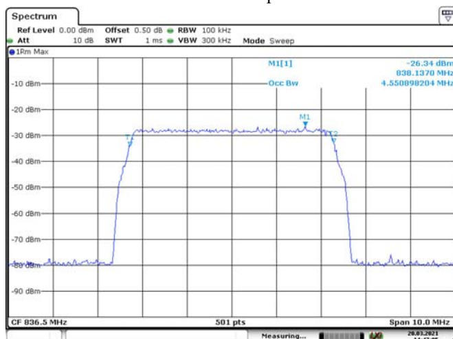
WCDMA-Input
