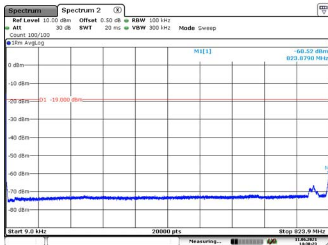
Cellular Band-1
