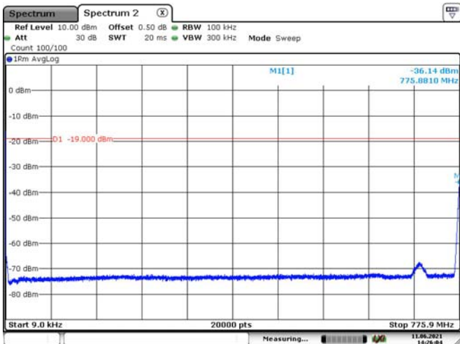
Upper 700M Band-1
