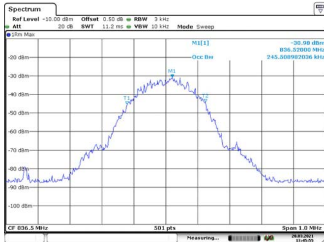
GSM-Input
