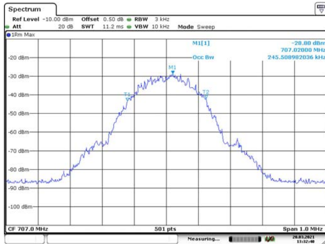
GSM-Input
