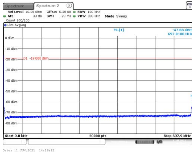
Lower 700M Band-1
