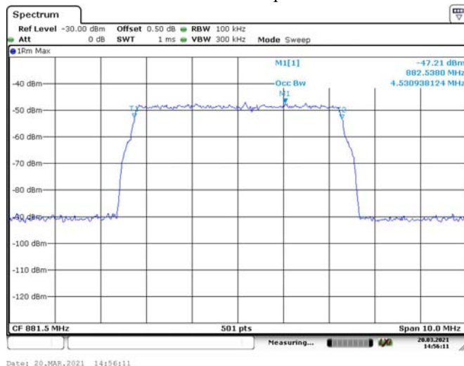
WCDMA-Input
