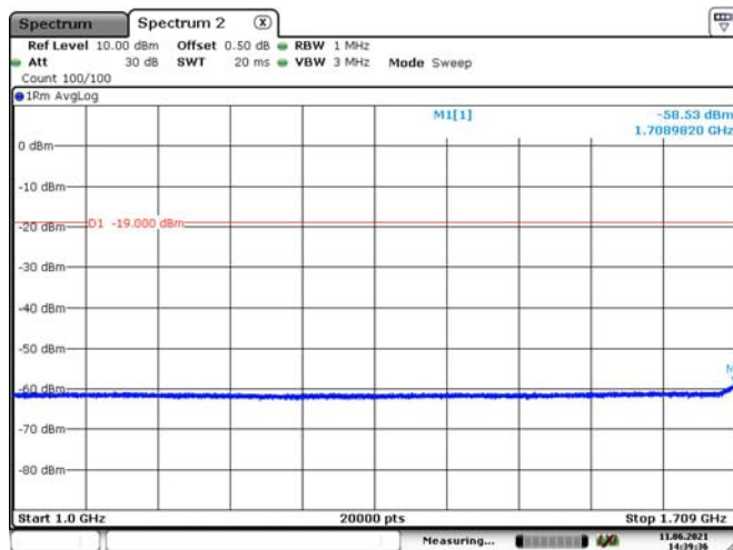
AWS Band-2
