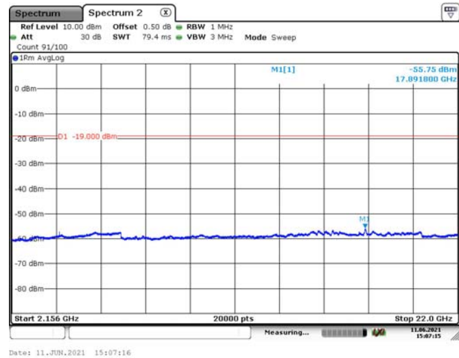
PCS Band-2
