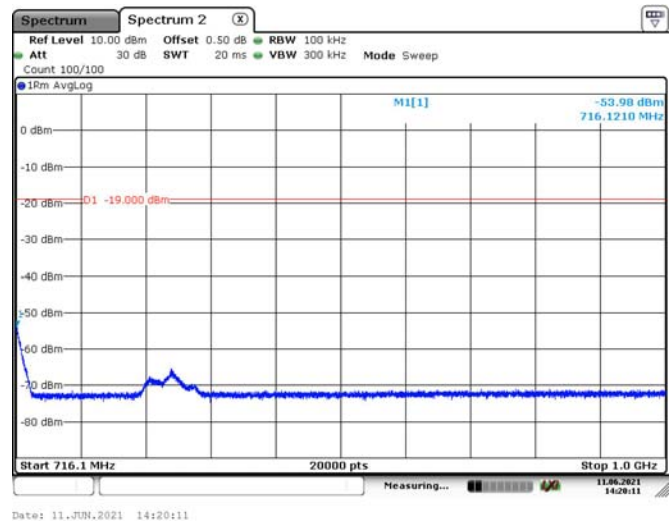
Lower 700M Band-2
