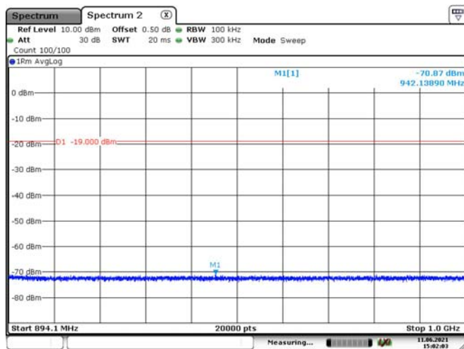
Cellular Band-2
