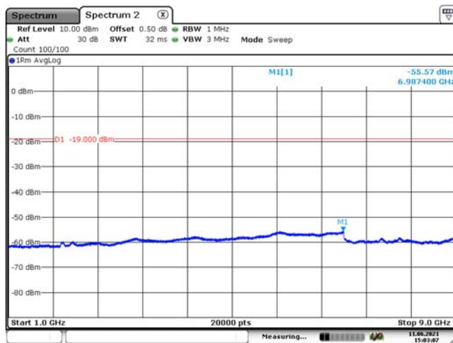
Cellular Band-3
