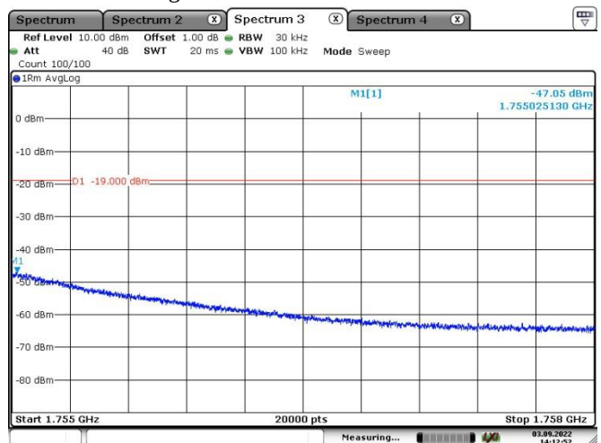
Right Side-CDMA-Above AGC
