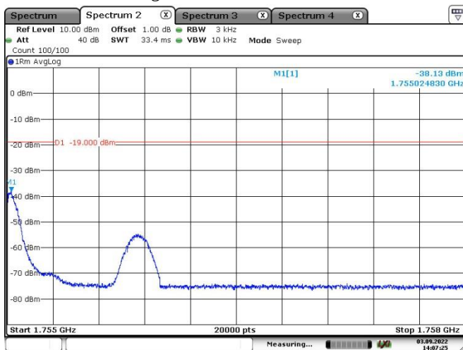
Right Side-GSM-Pre AGC
