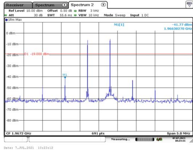
PCS Band Downlink -Pre AGC
