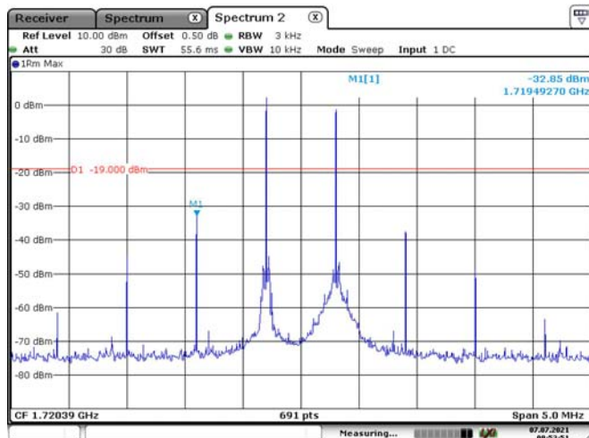
AWS Band Uplink-Above AGC
