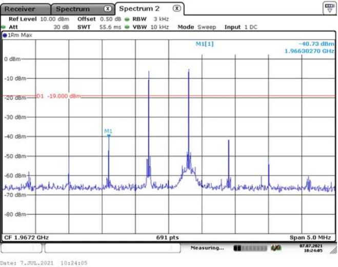
PCS Band Downlink -Above AGC
