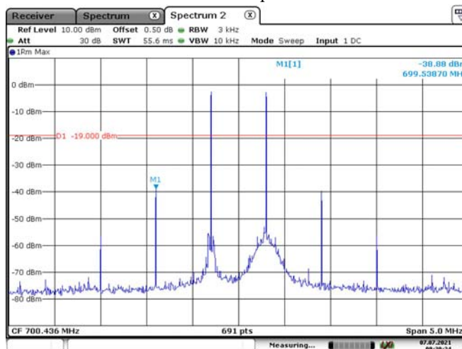
Lower 700MHz Band Uplink-Above AGC
