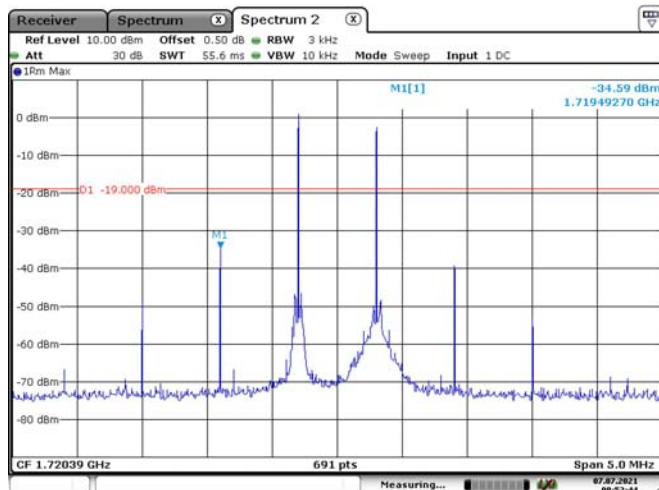
AWS Band Uplink-Pre AGC
