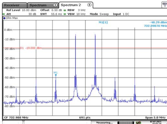
Lower 700MHz Band Downlink -Above AGC
