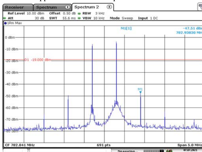
Upper 700MHz Band Uplink-Above AGC
