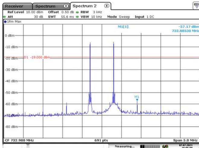
Lower 700MHz Band Downlink-Pre AGC
