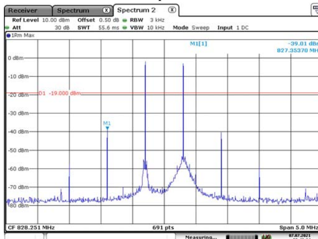
Cellular Band Uplink-Above AGC
