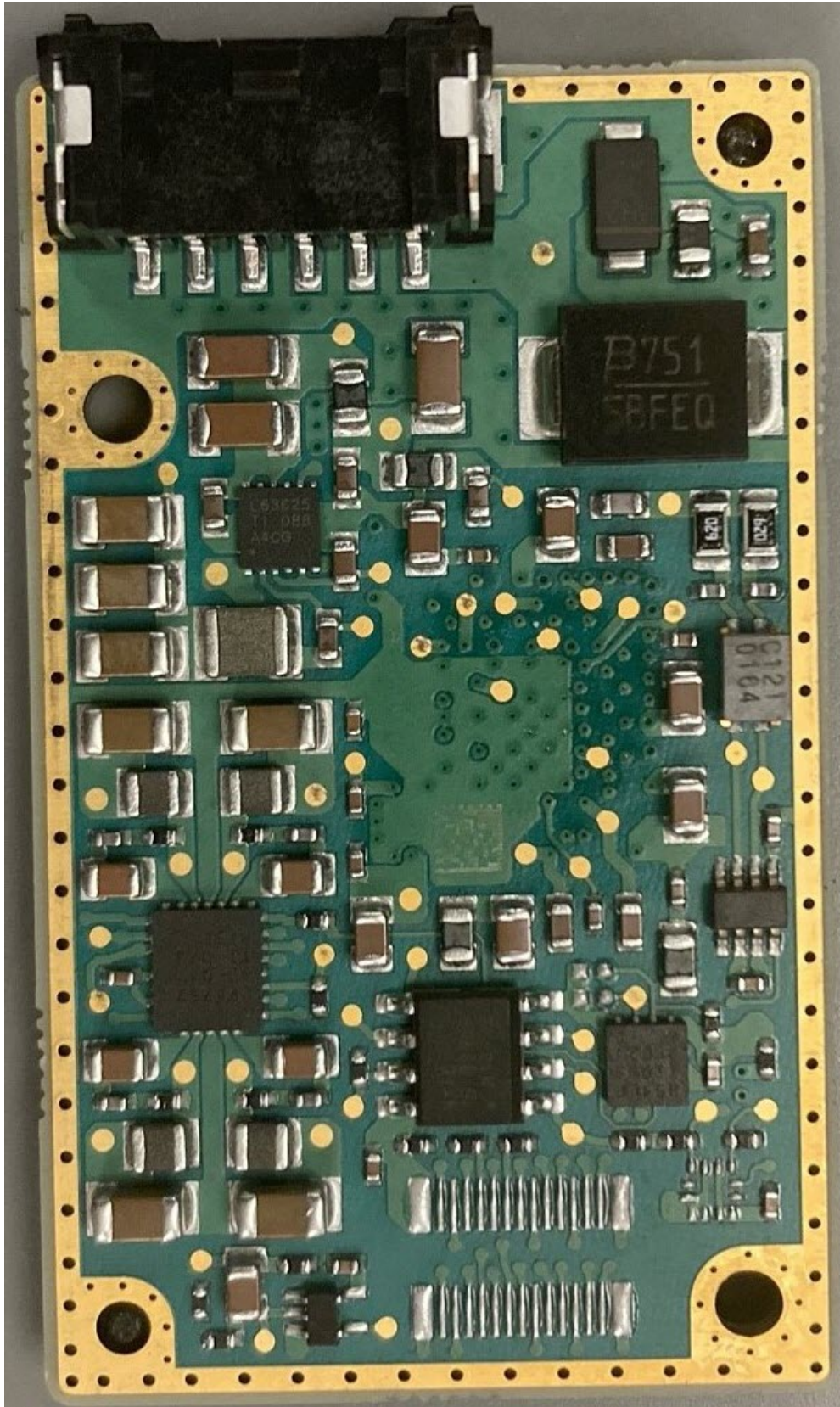
Figure 1: Top View
