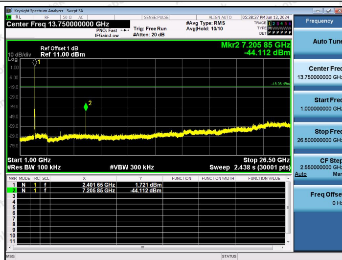
2.4G-Ant1-2402-1000~26500-PASS
