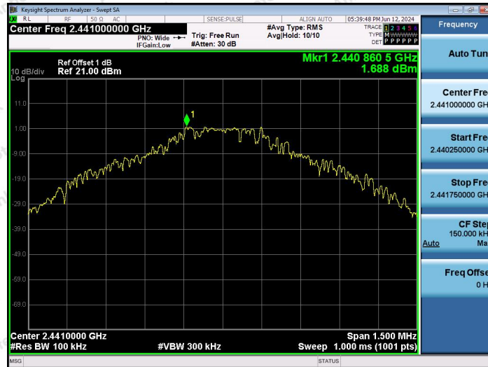
2.4G-Ant1-2441-0~Reference-PASS
