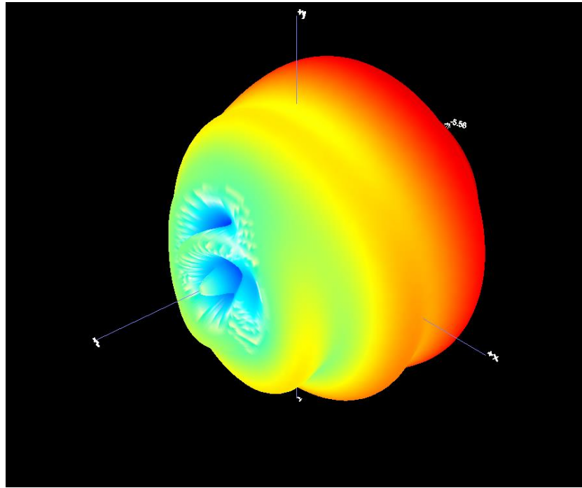
B1.1 3D Pattern for 611.8MHz
