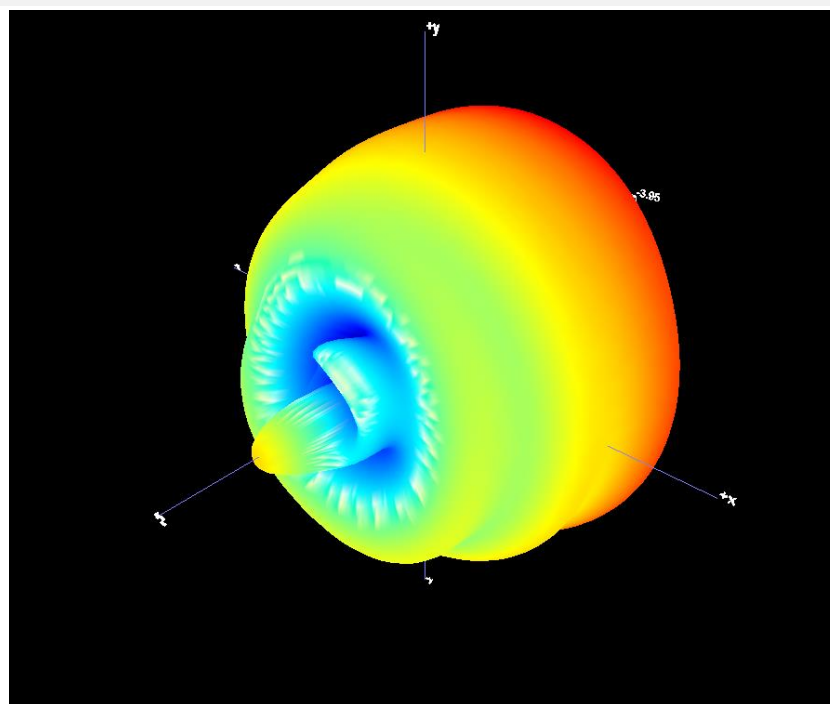
B1.3 3D Pattern for 626.8MHz
