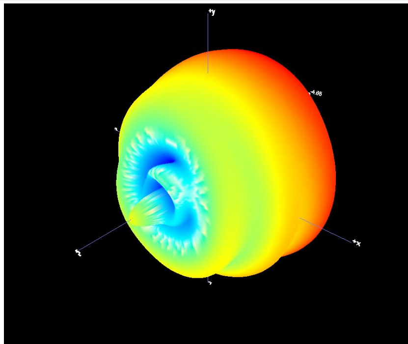
B1.2 3D Pattern for 621.8MHz
