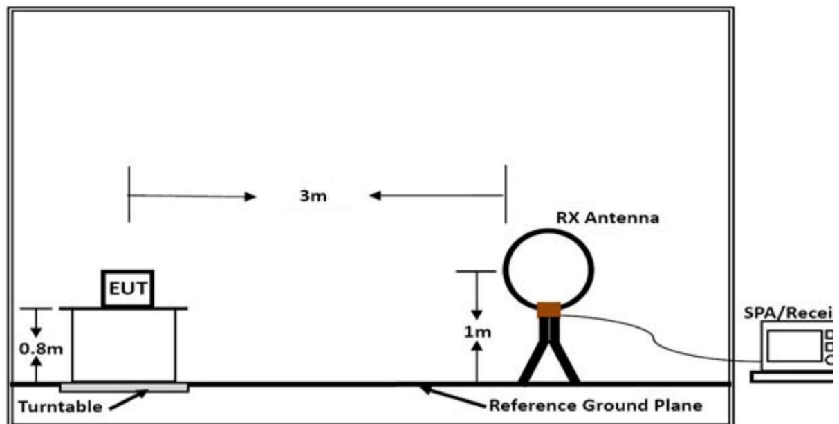
Figure 1. Below 30MHz
