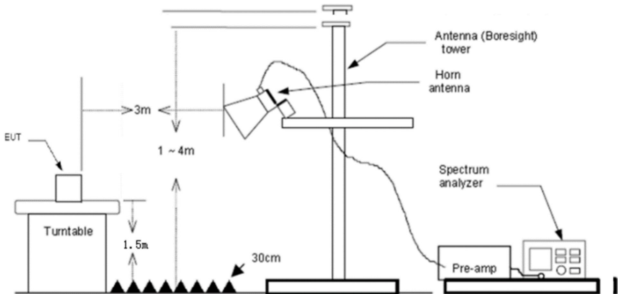
Figure 3. Above 1 GHz
