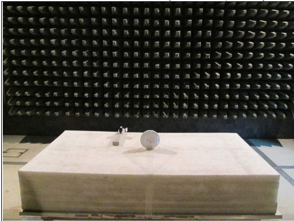
Radiated Emission Test below 1GHz (WLAN 2.4GHz, Mode A1)
