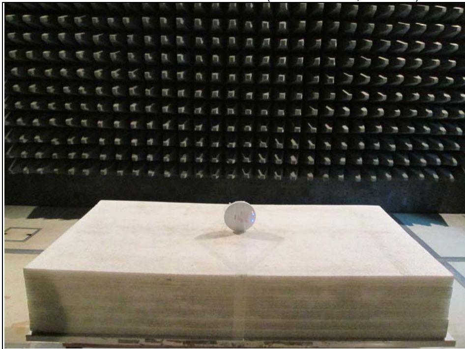
Radiated Emission Test below 1GHz (WLAN 2.4GHz, Mode A2)
