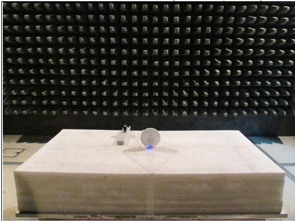
Radiated Emission Test below 1GHz (WLAN 5GHz, Mode A1)
