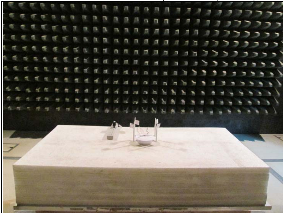
Radiated Emission Test below 1GHz (WLAN 2.4GHz, Mode B1)
