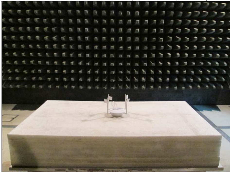
Radiated Emission Test below 1GHz (WLAN 2.4GHz, Mode B2)
