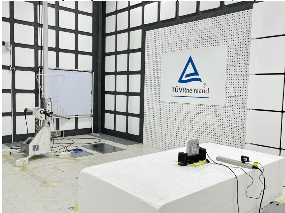
Photograph 4: Test Setup for Spurious Emissions (Back View 2, Adapter Mode)
