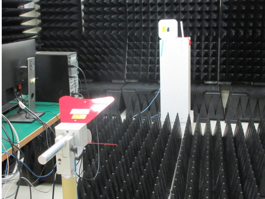
Photograph 17: Test Setup for DFS Mode (View 1)
