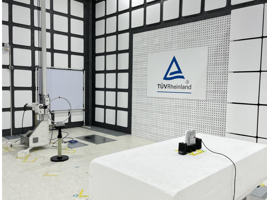
Photograph 11: Test Setup for Spurious Emissions (Back View 1, POE Mode)
