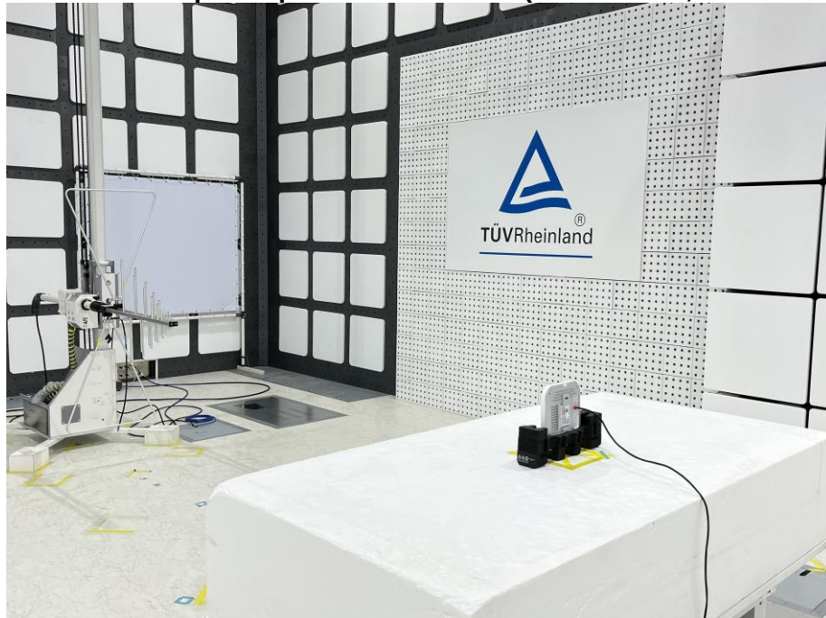
Photograph 12: Test Setup for Spurious Emissions (Back View 2, POE Mode)
