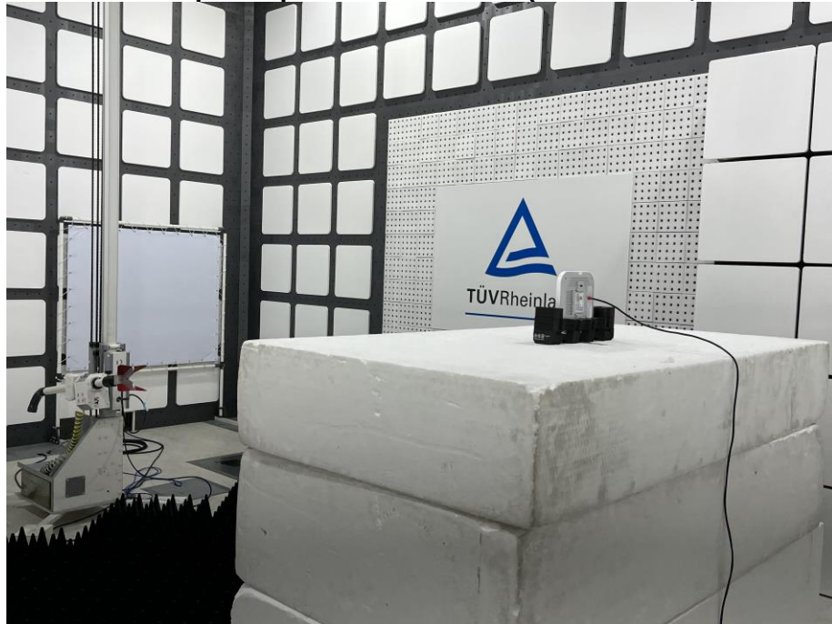
Photograph 13: Test Setup for Spurious Emissions (Back View 3, POE Mode)
