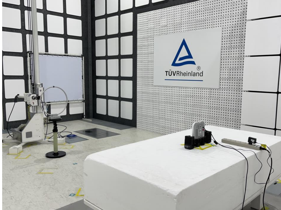
Photograph 3: Test Setup for Spurious Emissions (Back View 1, Adapter Mode)
