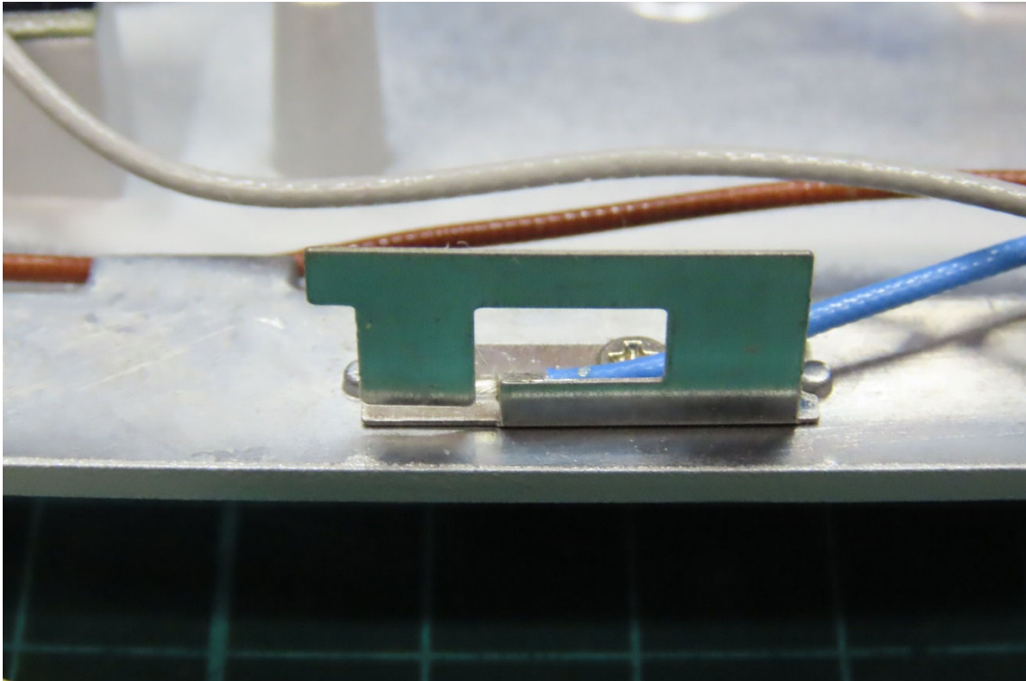
(23) EUT Photo_5GHz-1 Antenna
