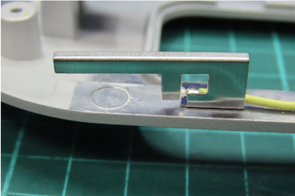
(19) EUT Photo_2.4GHz-3 Antenna
