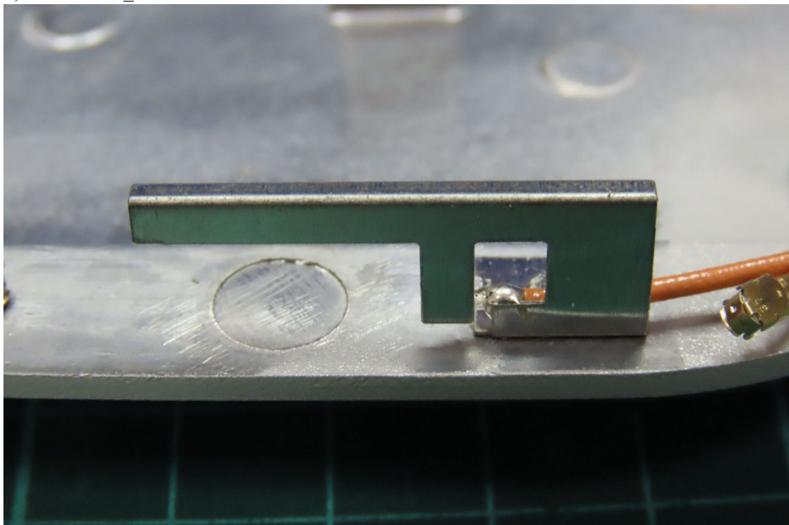
(14) EUT Photo_2.4GHz-1 Antenna
