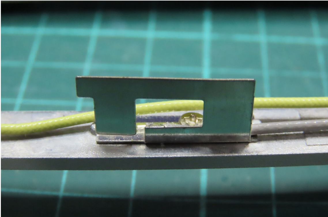
(25) EUT Photo_5GHz-2 Antenna
