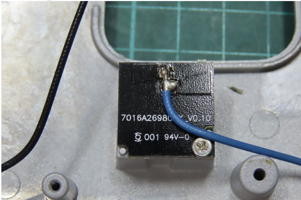
(33) EUT Photo_6GHz-4 Antenna
