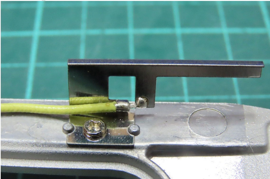
(18) EUT Photo_2.4GHz-3 Antenna
