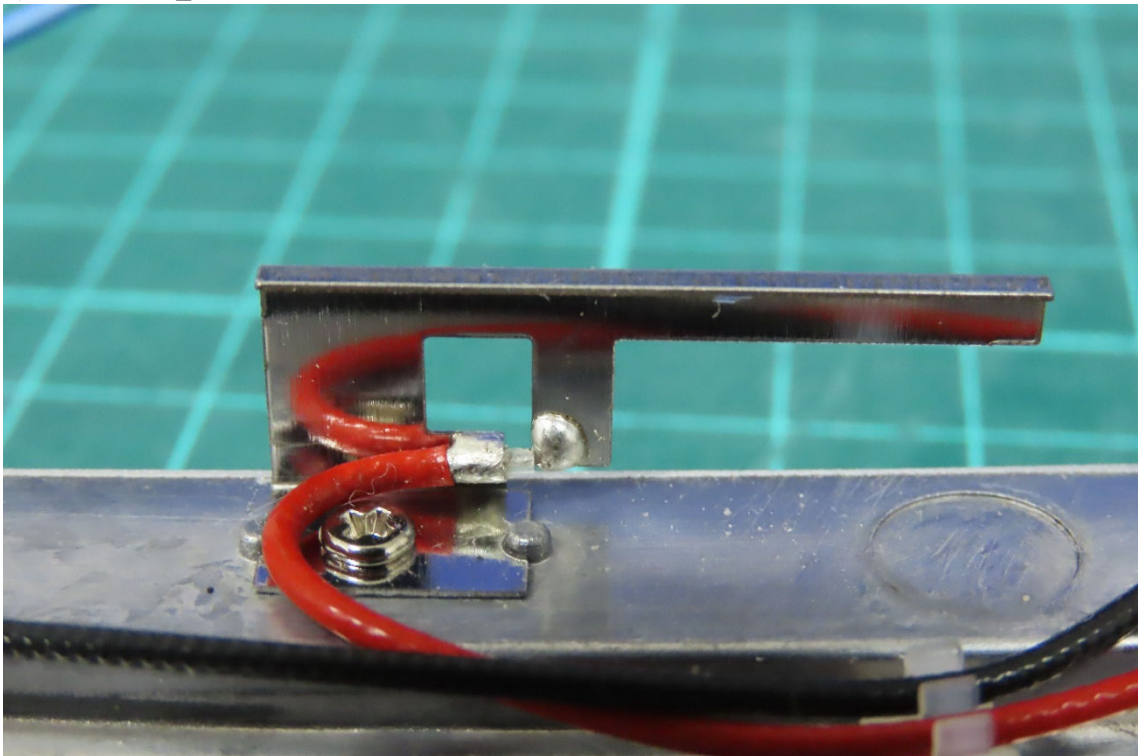
(20) EUT Photo_2.4GHz-4 Antenna
