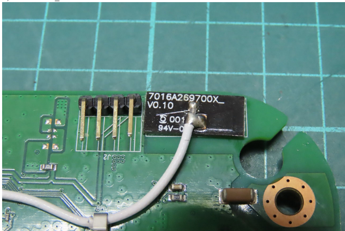
(31) EUT Photo_6GHz-2 Antenna
