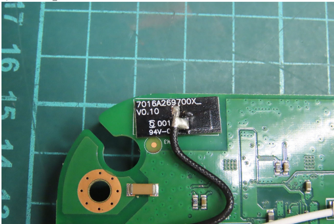
(30) EUT Photo_6GHz-1 Antenna
