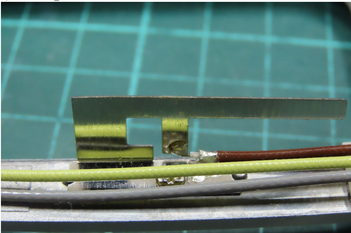
(16) EUT Photo_2.4GHz-2 Antenna
