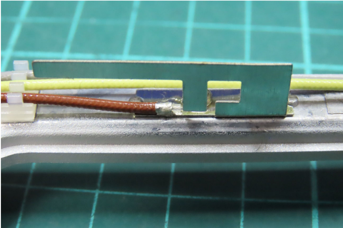
(17) EUT Photo_2.4GHz-2 Antenna
