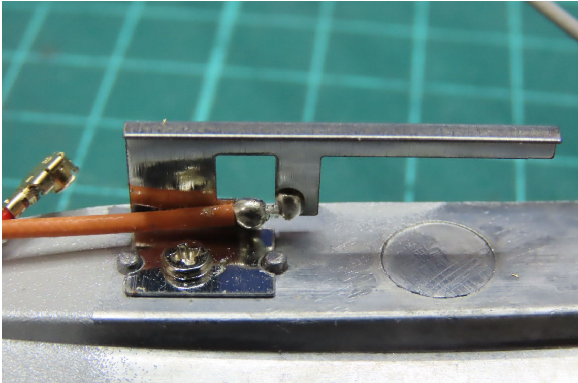
(15) EUT Photo_2.4GHz-1 Antenna
