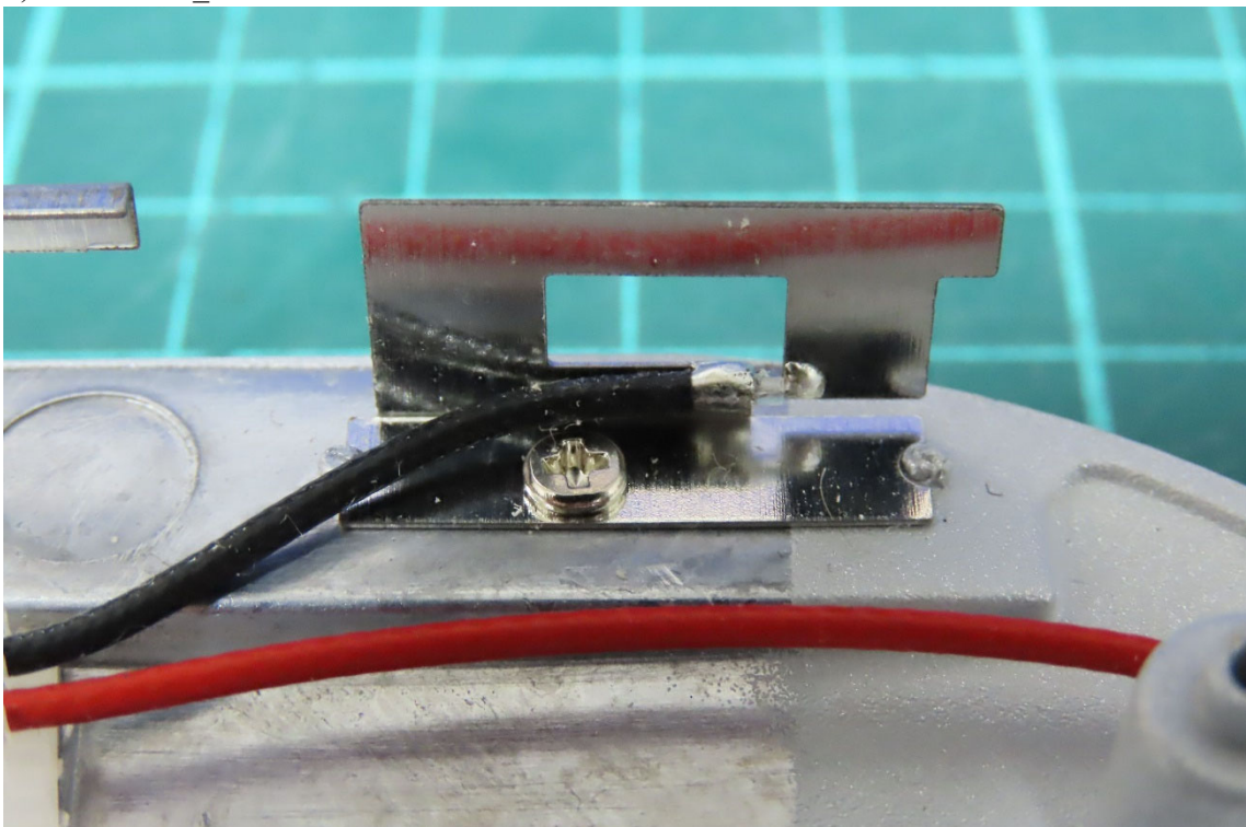
(28) EUT Photo_5GHz-4 Antenna
