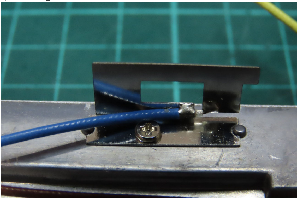
(22) EUT Photo_5GHz-1 Antenna
