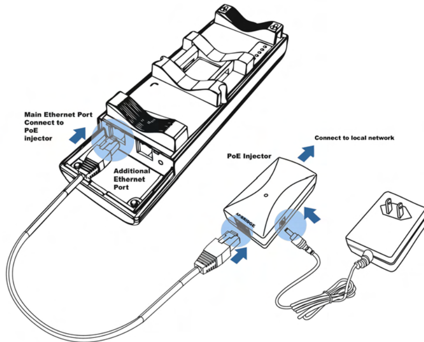
Figure 2-1: Installing the ENH202
