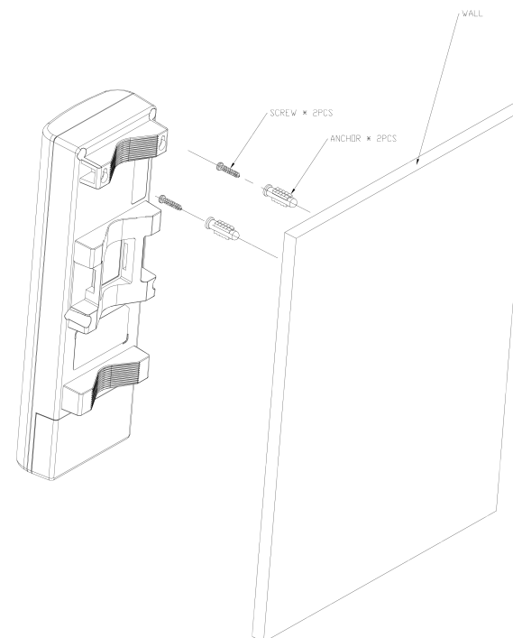
Figure 2-2: Wall Mounting the ENH500
