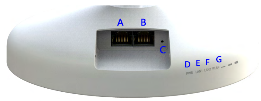
Figure 1-1: Back Panel View
