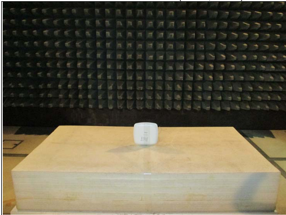
Radiated Emission Test below 1GHz (2.4GHz, Mode B)
