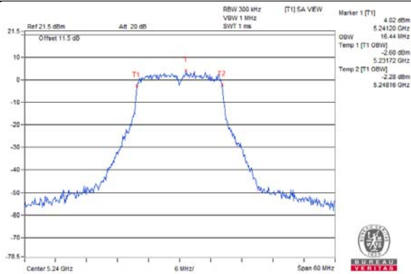
802.11ax (HT20) / Chain 0 / CH 48
