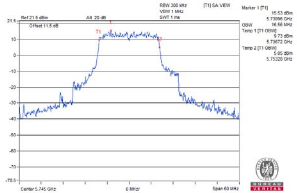
802.11ax (HT20) / Chain 1 / CH 149
