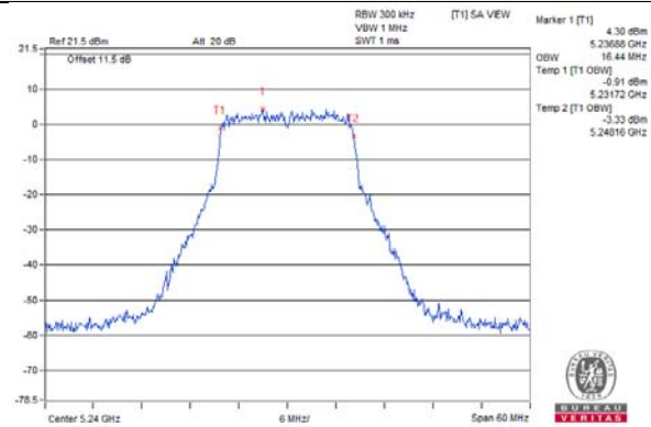
802.11ax (HT20) / Chain 1 / CH 48
