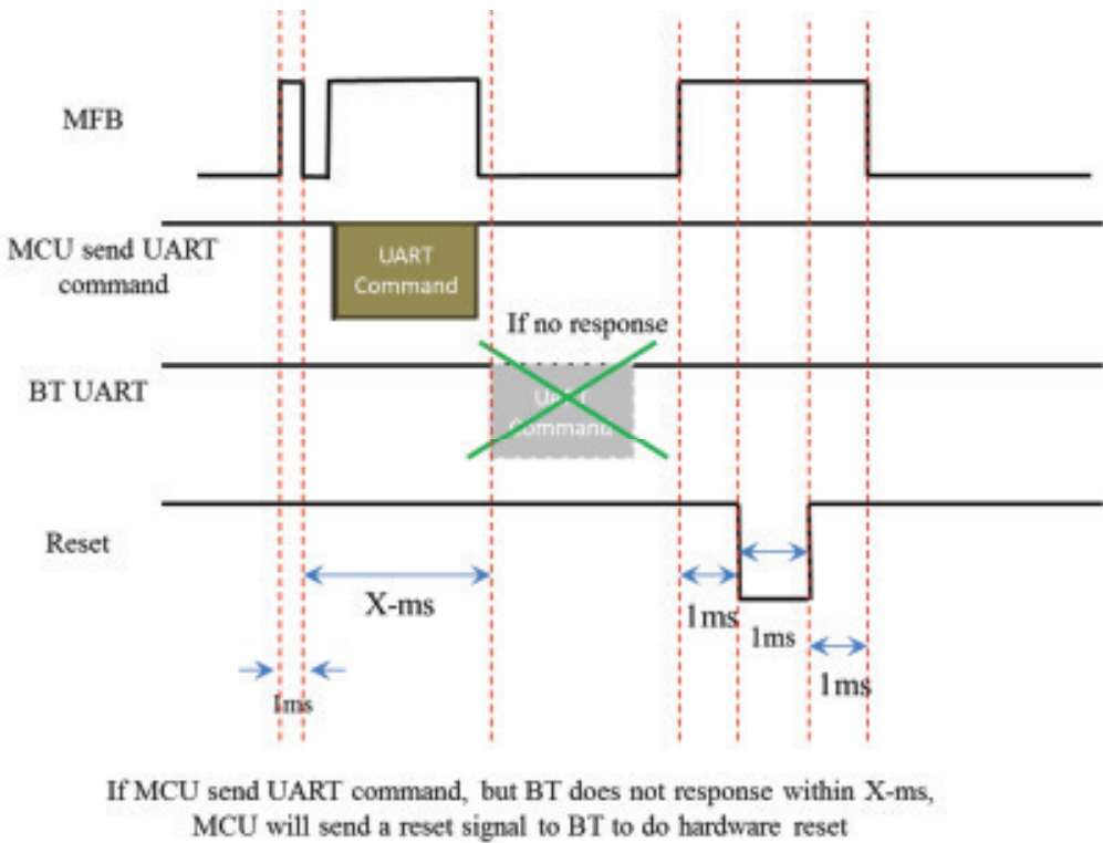
FIGURE 2-6: RESET TIMING SEQUENCE IF MODULE HANGS UP
