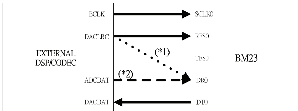
FIGURE 2-10: SLAVE MODE REFERENCE CONNECTION
