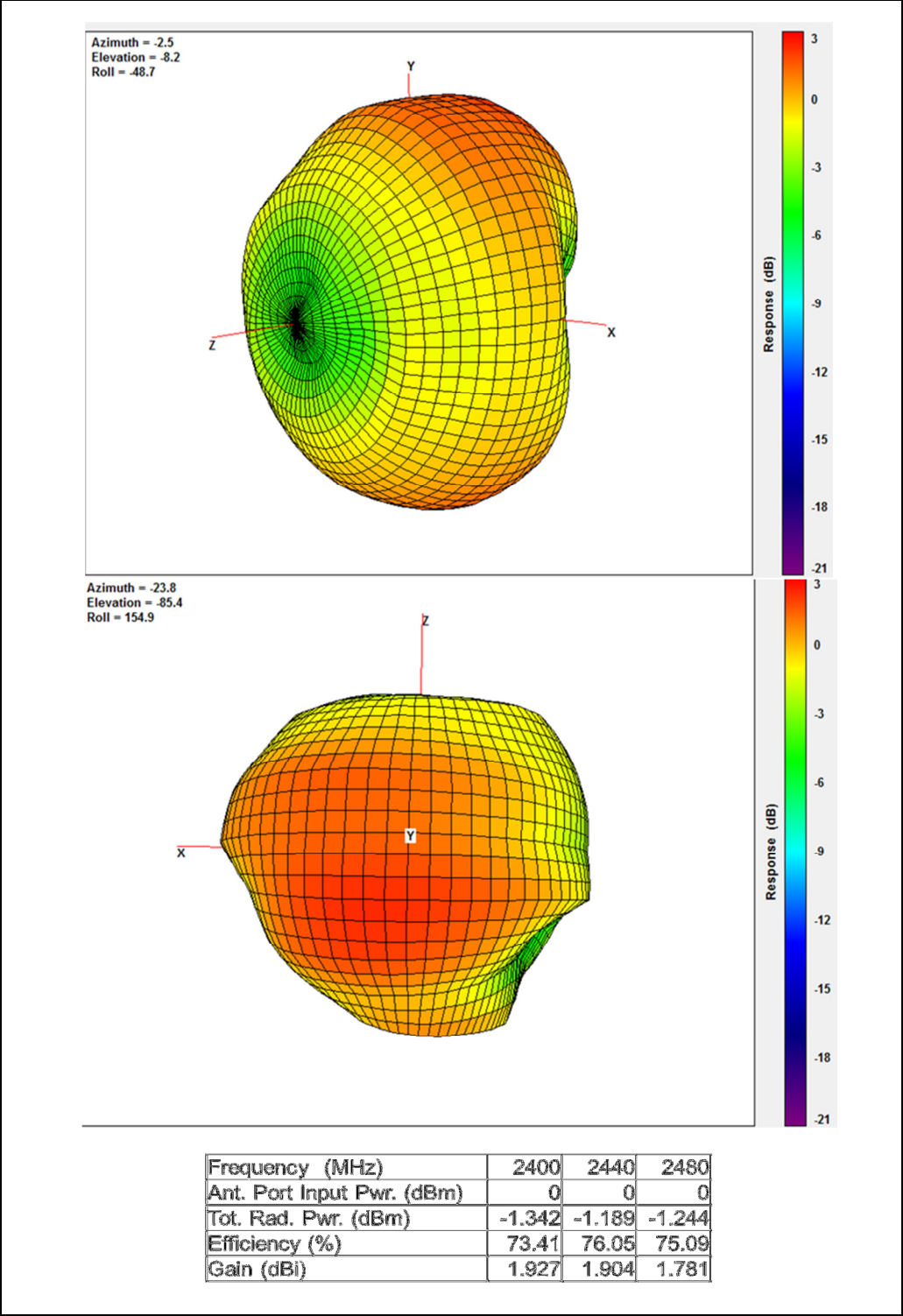
FIGURE 1-1: BM64 ANTENNA RADIATION PATTERN
