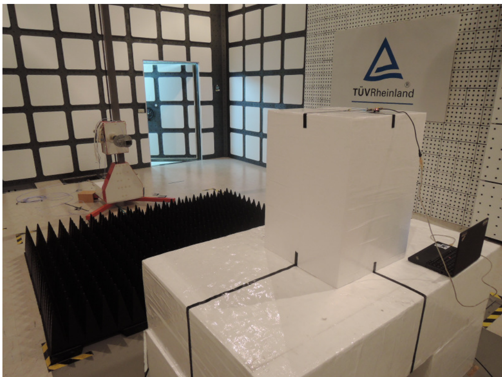
Photograph 5: Set-up for Spurious Emissions (IC)
