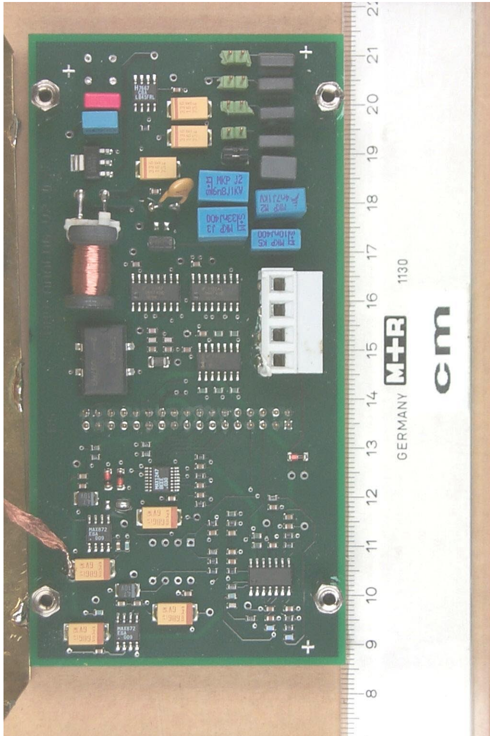
20353_5.jpg METT HHU 76519 RF unit, analogue board, top view
