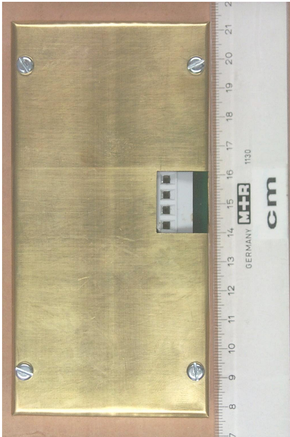
20353_9.jpg METT HHU 76519 shielding of the RF unit, top view
