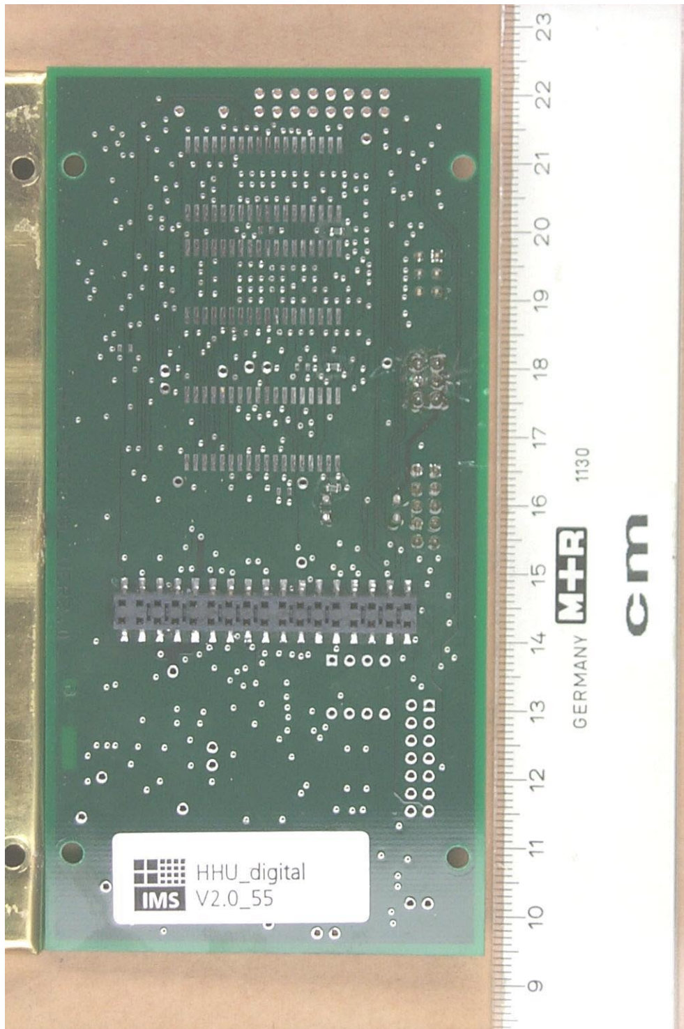
20353_7.jpg METT HHU 76519 RF unit, digital board, bottom view
