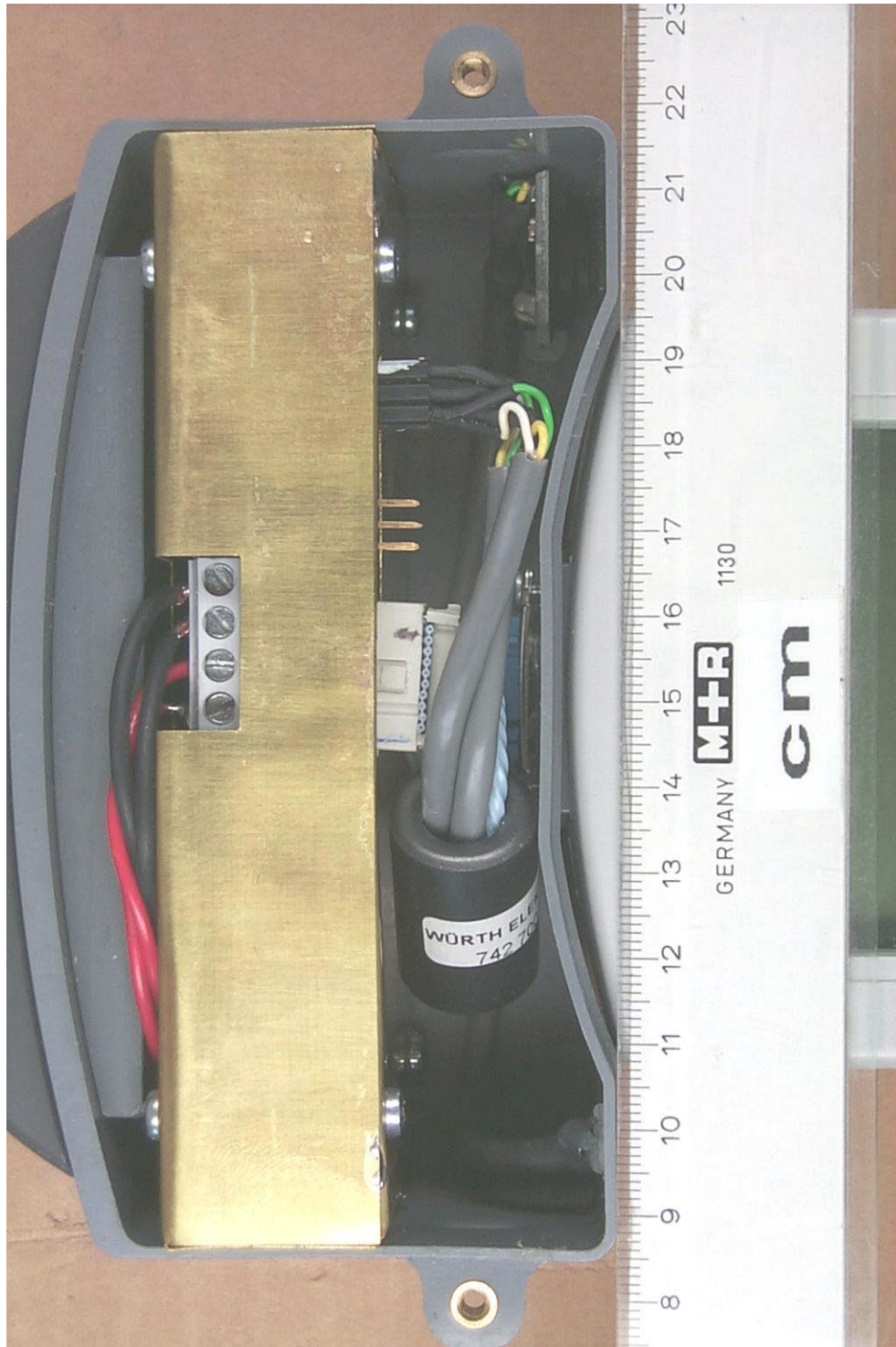
20353_4.jpg METT HHU 76519 internal view RF unit
