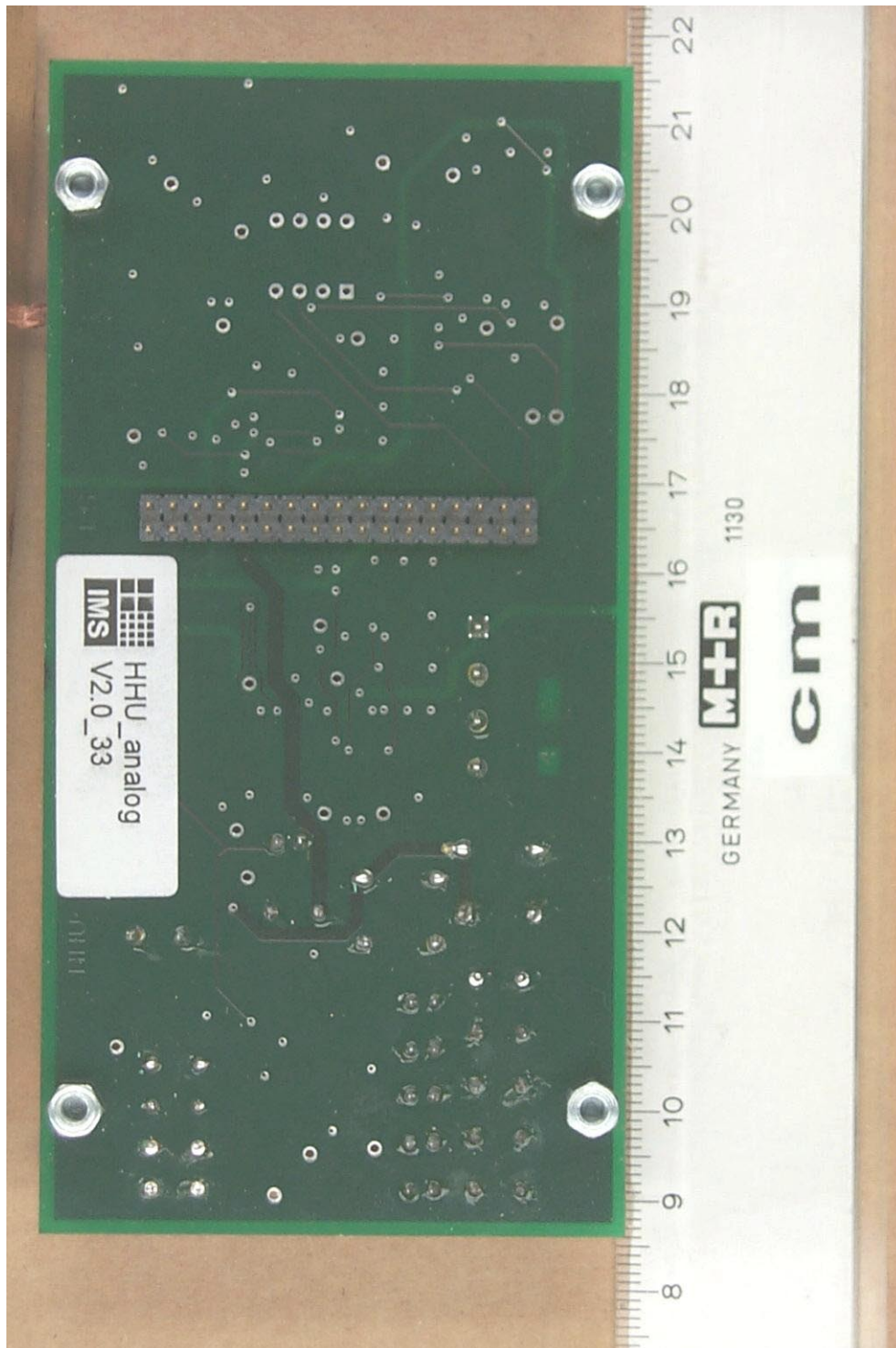
20353_10.jpg METT HHU 76519 RF unit, analogue board, bottom view
