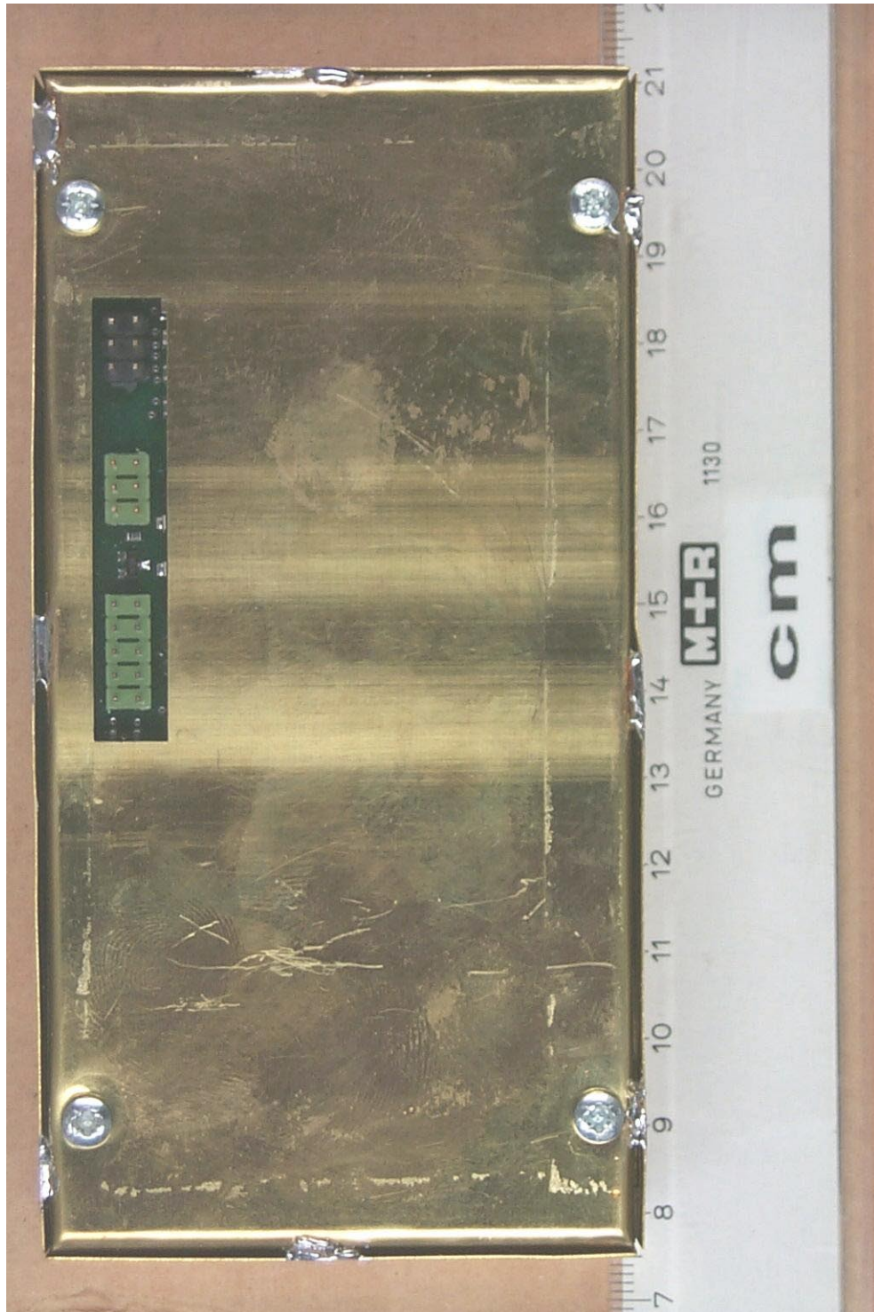
20353_6.jpg METT HHU 76519 shielding of the RF unit, bottom view
