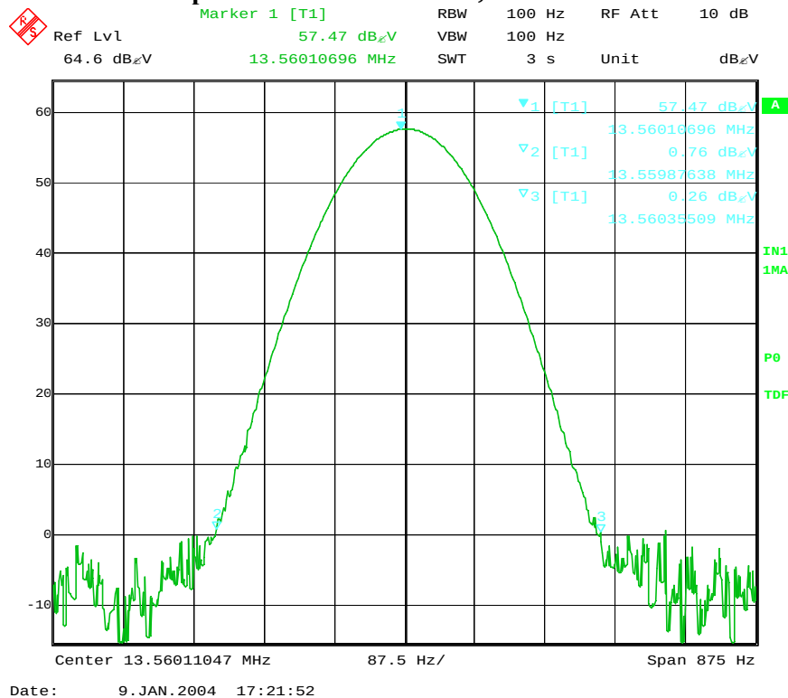
Graph # 7: In Band Emission, RBW = 100 Hz
