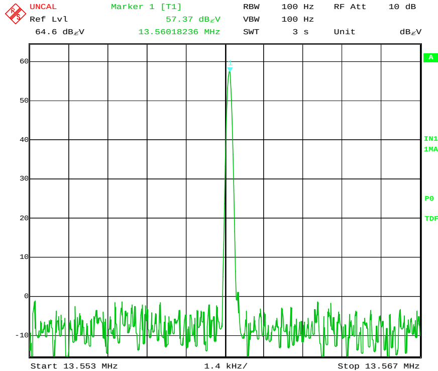
Graph # 7: In Band Emission, RBW = 100 Hz
