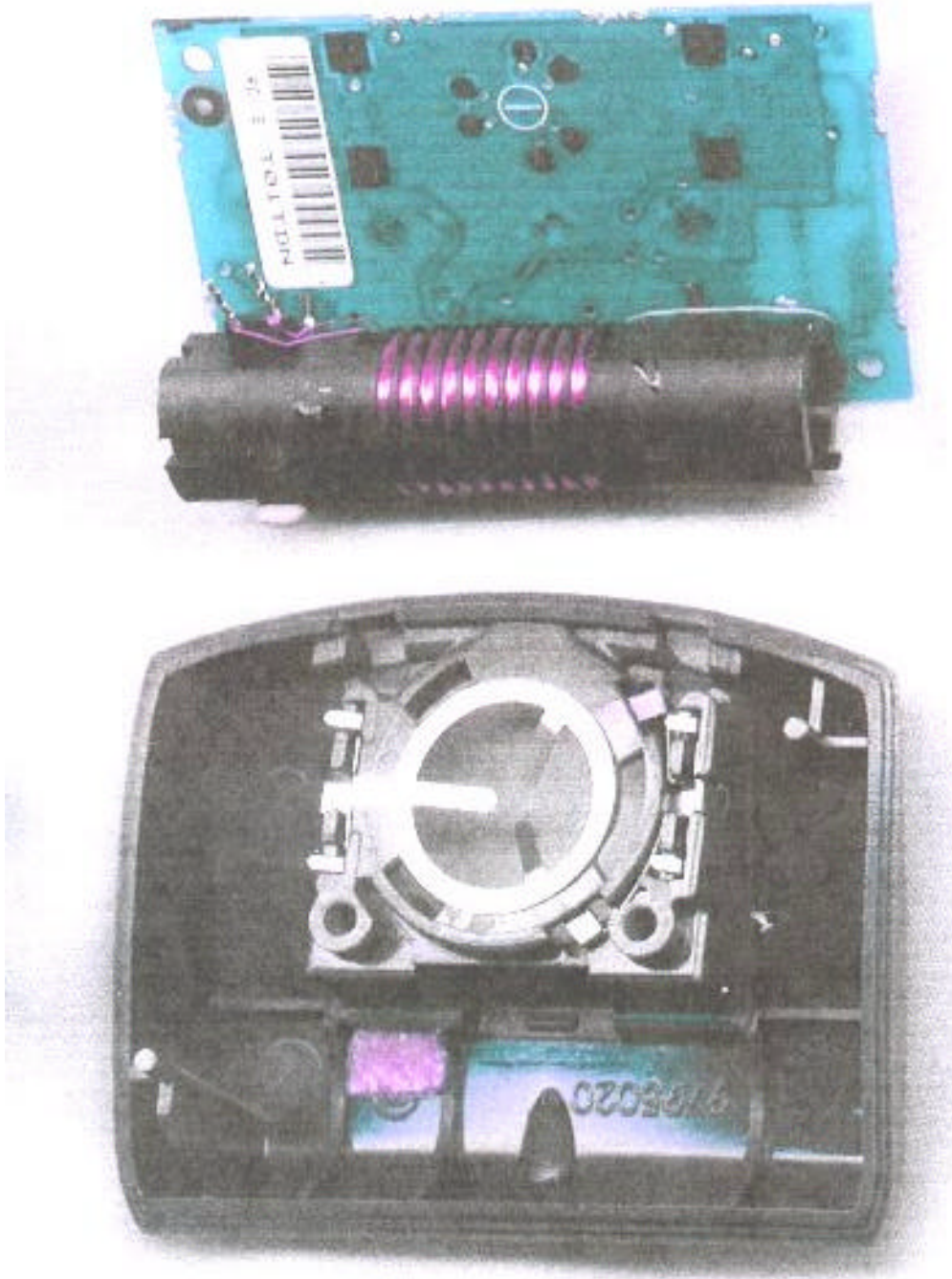
Fig 5. Transponder PCB Assembly Bottom
