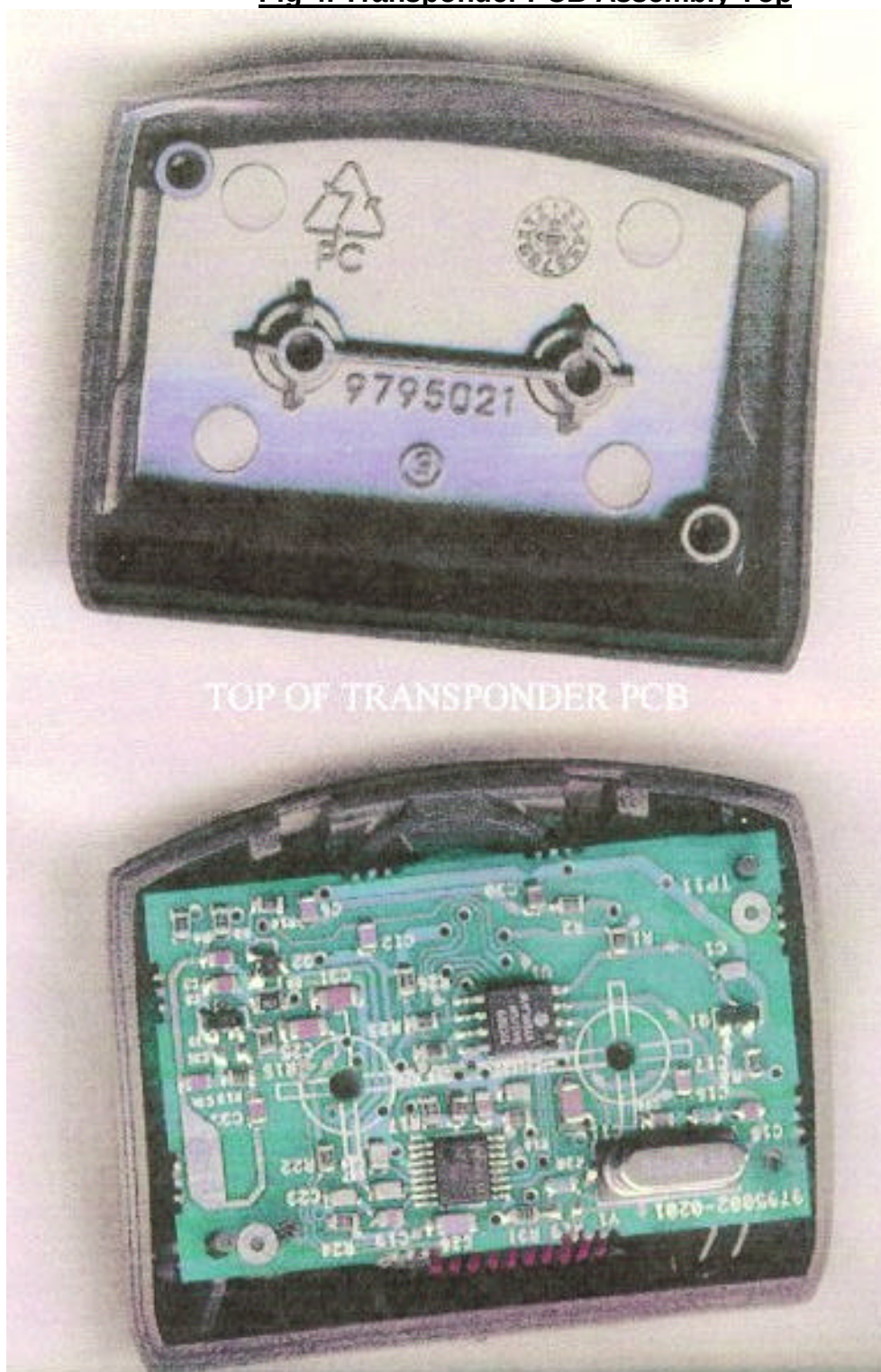
Fig 4. Transponder PCB Assembly Top
