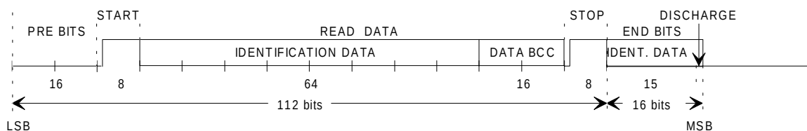
Figure 15: R/W Read Data Format
