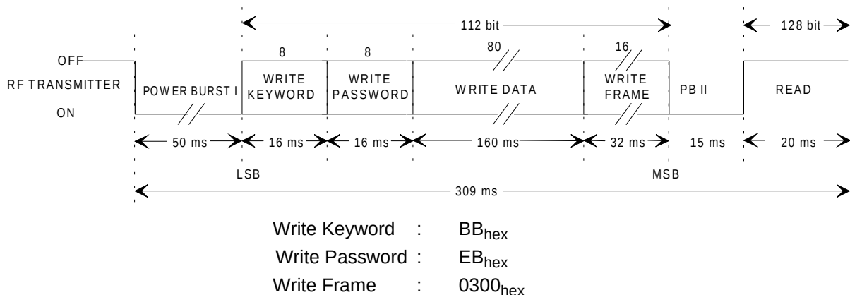
Figure 7: Programming Data Format of the 64-bit Read/Write Transponder
