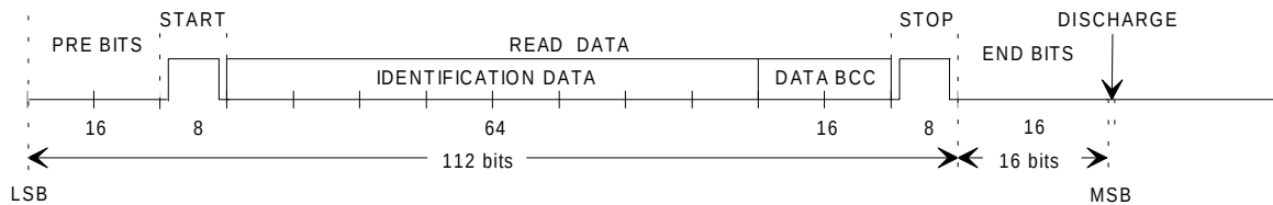
Figure 14: RO Read Data Format
