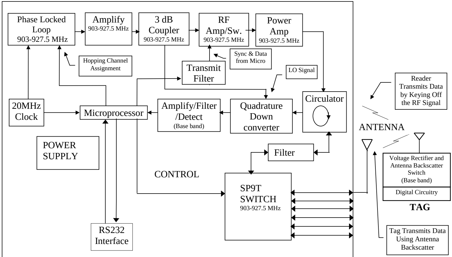
Tag-it UHF Reader (RI-RU1-001A-00) Functional Block Diagram
