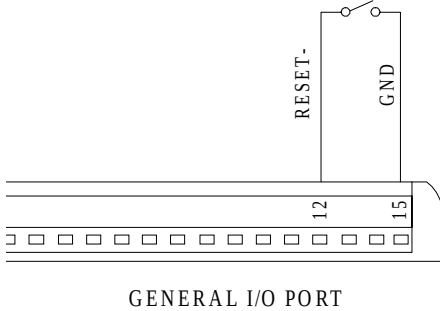
Figure 15: RESET Push-button Wiring
