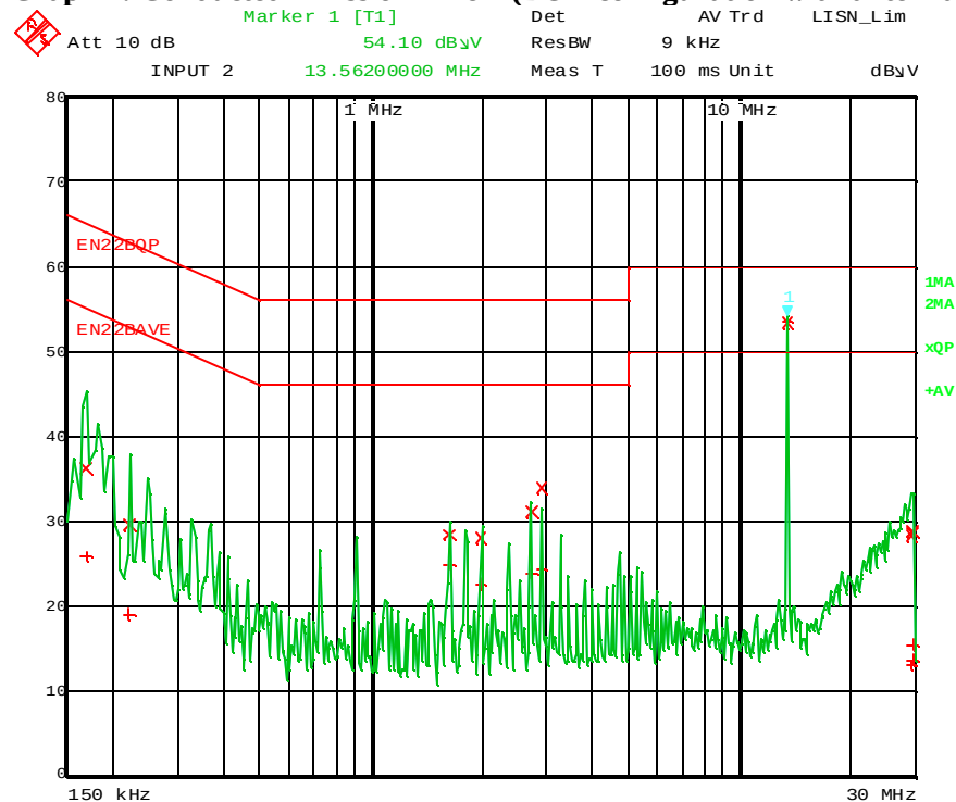
Graph 2: Conducted Emission Line 2 (BOX configuration with antenna)
