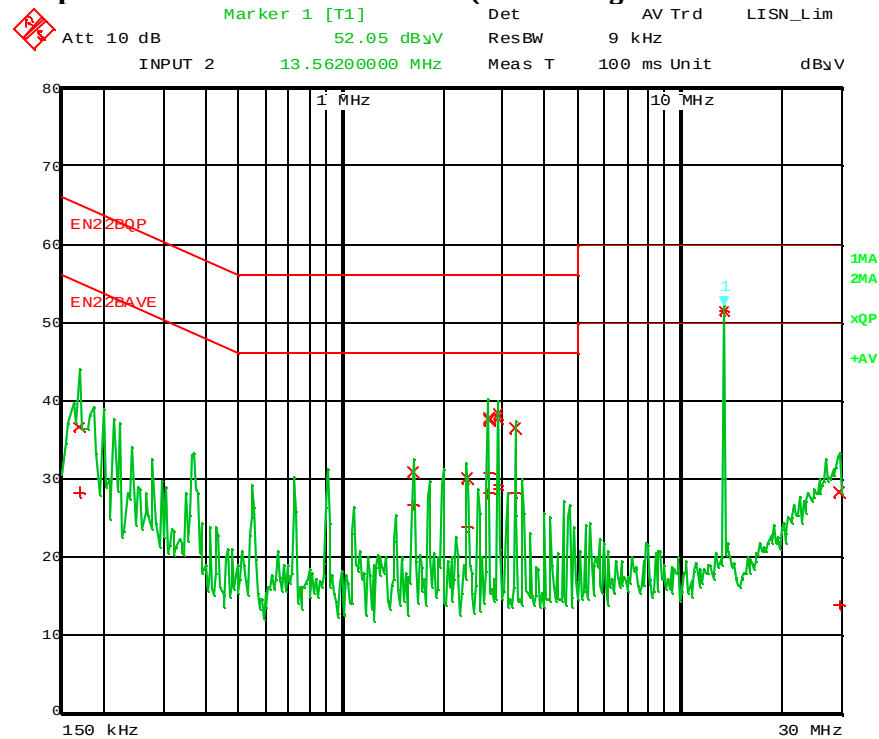
Graph 1: Conducted Emission Line 1 (BOX configuration with antenna)
