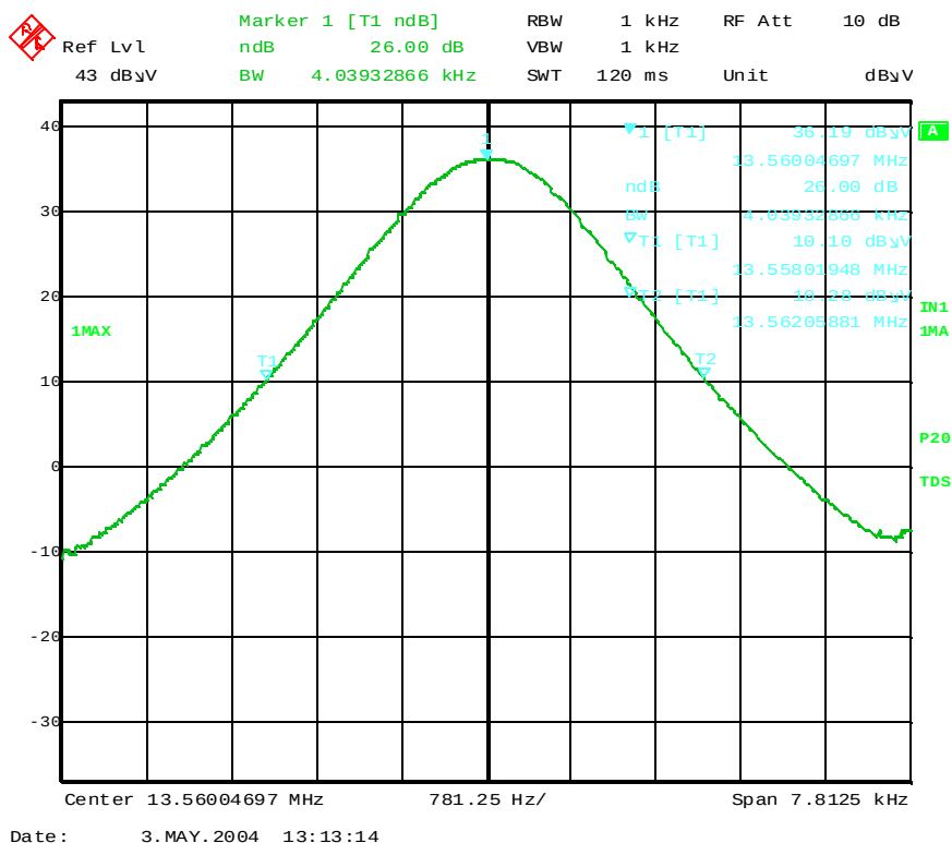
Graph # 9: 26 dB Bandwidth in In-Band Emission, RBW = 1 kHz
