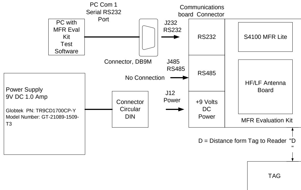
Figure 4: Hardware Set Up MFR Evaluation Kit
