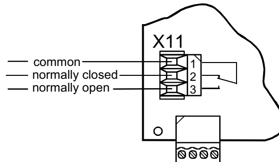
Figure 8: Relay Connector
