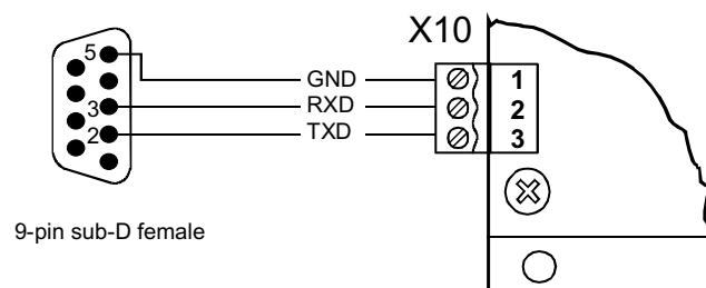
Figure 10: RS232 Interface
