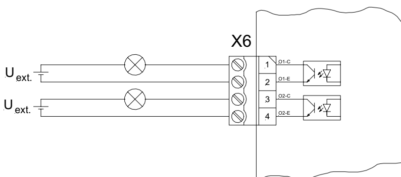
Figure 7: Optocoupler Outputs
