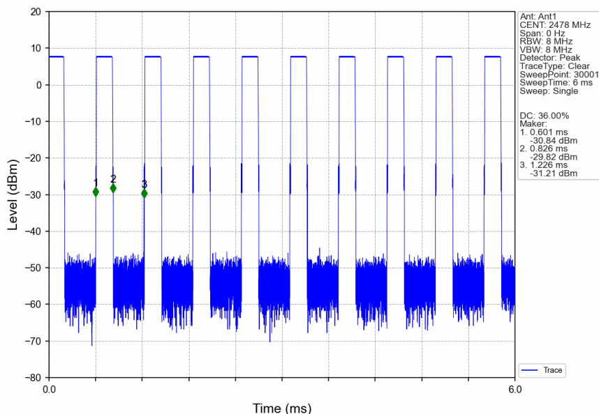
2M_HCH_2478MHz_Ant1_NTNV
